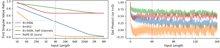
Figure 7: Expected RoPE behavior for our proposed method and three baselines. Dotted line indicates hypothetical training length of 4k and head dimension is 128. Left: Repeats the Fig. 4 singular value ratio before/after RoPE, for a synthetic point cloud of ones vectors. Right: Long-term RoPE decay for the same techniques, showing similar behaviors.
