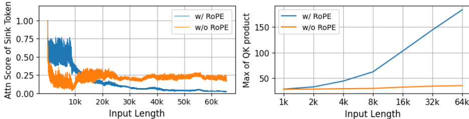
Figure 6: Left: Sink token attention weight vs. input length. With RoPE, sink-token attention decays to zero beyond the training length; without RoPE it remains stable. Right: Maximum Query–Key dot product vs. input length. The max QK product increases with length only when RoPE is active.
