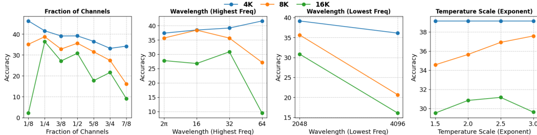
Figure 12: Llama 1B ablation studies with average RULER scores on the y-axis. The x-axis of the 4 plots cover fraction of channels, wavelength (high frequency), wavelength (low frequency) and temperature scaling, respectively. The color coded legend represents context lengths 4k, 8k and 16k.
