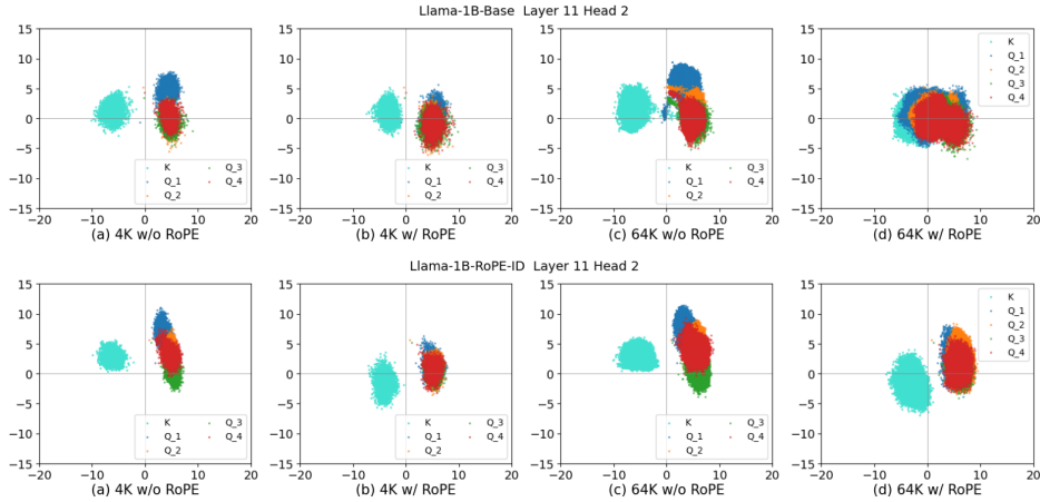
Figure 14: Clustering behavior for our trained models. Vanilla transformer (top) matches prior LLM observations; RoPE-ID (bottom) maintains stable cluster separation.
