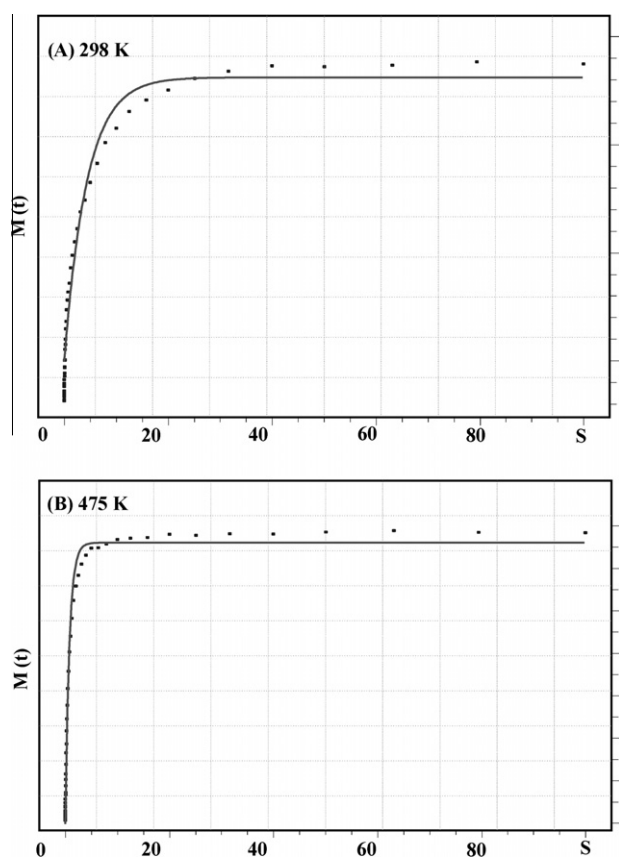
Fig. 5. ^1\text{H} saturation-recovery data for the ^{15}\text{N} -enriched IRMOF-3 at 298 K (A) and at 475 K (B) plotted in arbitrary units. The smooth line in each is a fit to a single-exponential recovery.
