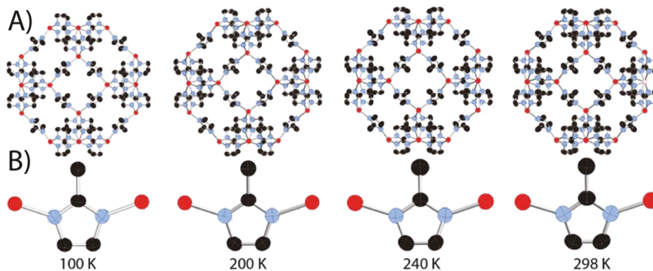
Figure 2. (a) ORTEP representation (50% probability) of sod unit of ZIF-8 at 100, 200, 240, and 298 K. (b) ORTEP representation (50% probability) of imidazolate unit of ZIF-8 at 100, 200, 240, and 298 K. Zinc (red), nitrogen (blue), and carbon (black).
