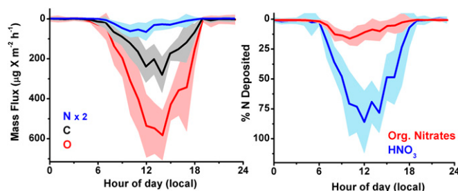
Fig. 8. ( Left ) Net carbon, oxygen, and nitrogen downward flux by mass, calculated from molecular formulas for compounds shown in SI Appendix, Table S1 , and averaged over the dates in the study. ( Right ) Percent contribution of organic nitrates and nitric acid to the measured oxidized nitrogen flux.
