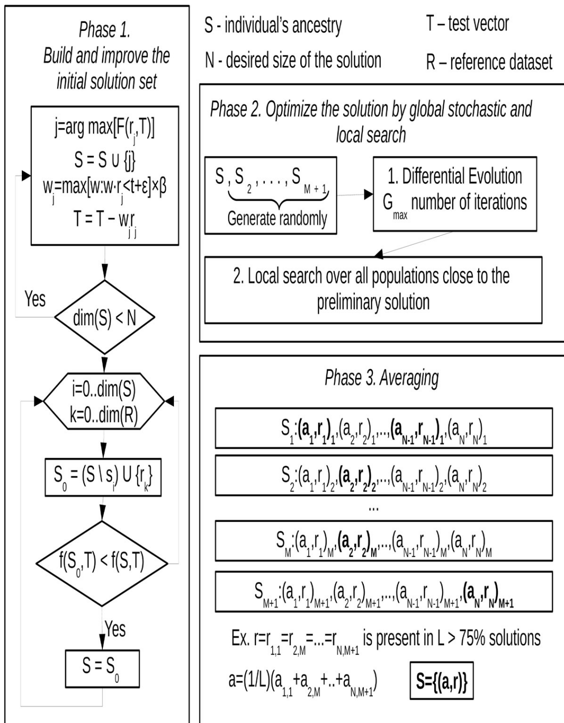
Figure 2 Flowchart of reAdmix .
