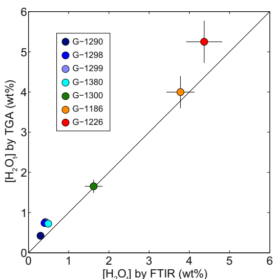
Fig. 4. Comparison of the concentration of water, [\text{H}_2\text{O}_\text{l}] , measured by TGA and by FTIR (corresponding values provided in Table 4). We attribute the slightly higher water contents measured by TGA predominantly to the adsorption of atmospheric water.
