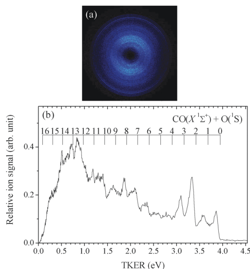
Fig. 5 (a) Time-sliced velocity-mapped raw image of \text{O}^+ and (b) total kinetic energy release (TKER) spectrum of the photofragments CO and O from photodissociation of \text{CO}_2 at 13.589 eV. The VUV laser was set at 109\,596.7\text{ cm}^{-1} to coincide with \text{O}(^1\text{S}) transition 2s^22p^3(^2\text{P}^\circ)4d\ ^1\text{P}^\circ \leftarrow 2s^22p^4\ ^1\text{S} .
