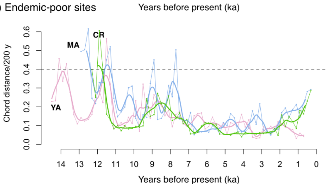
Figure 2. Palynological rate of change at two sites within (a) endemic-rich vegetation zones (Wentworth and Moose) and (b) three endemic-poor vegetation zones (Yahoo, Martins, and Crocker). Pollen assemblages were interpolated to 200-year intervals and the chord distance was calculated between assemblages across each time interval. The smoothed line is a LOESS fit in 500-year windows. Dashed lines show the general criterion for assessing vegetation analogs, suggesting that the endemic-poor sites were experiencing turnover at the scale of coarse vegetation zones within 200-year intervals.
