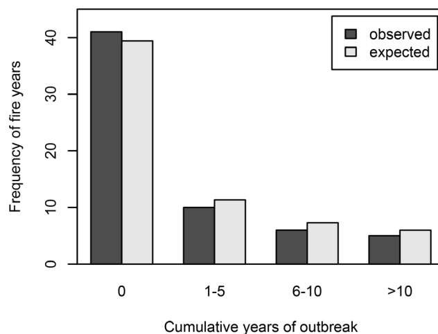
Fig. 8. Distribution of fire years by outbreak duration (cumulative number of years of western spruce budworm outbreak). Expected distribution is based on fires occurring randomly with respect to the timing of outbreaks.
