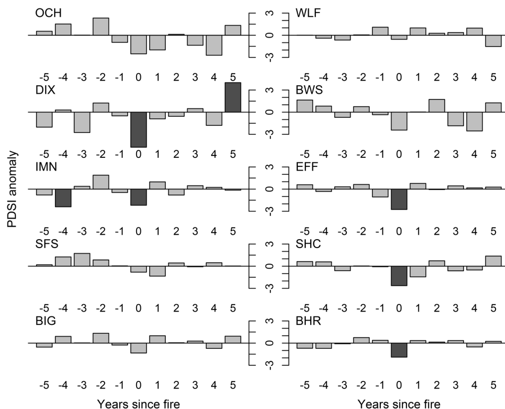
Fig. 4. Superposed epoch analysis indicating the direction of Palmer Drought Severity anomalies for an 11-year window centered on fire dates at each of our 10 sites. Descending bars indicate a negative association with PDSI (i.e., droughty conditions), ascending bars indicate a positive association with PDSI (i.e., wetter conditions). Dark grey shading shows statistically significant (at the 95% confidence interval) anomalies.
