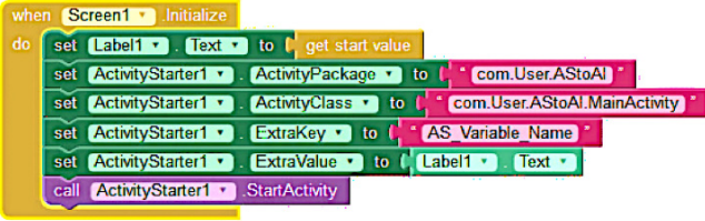
Figure 1. AI blocks to communicate with AS app.
