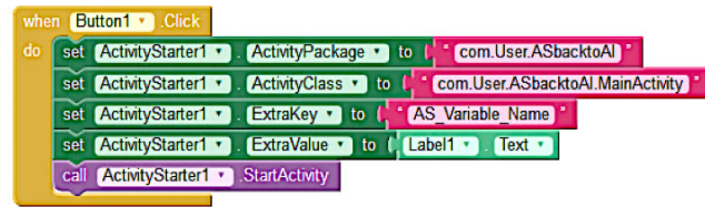
Figure 2. AI application intent for AS application.
