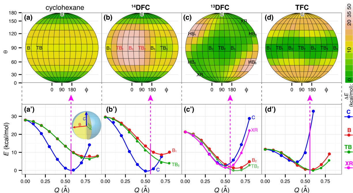
Figure 3. (a–d): Potential energy surface (PES) of cyclohexane, ^{14}\text{DFC} , ^{13}\text{DFC} , and TFC (as denoted on the plot) with respect to \theta and \phi at Q = 0.57 \text{ \AA} ( Q was obtained from the DFT calculations of parent cyclohexane in its chair conformation) [M06-2X/6-31G(d)+PCM( \text{CH}_2\text{Cl}_2 )]. Step size of 15^\circ was used for both \theta and \phi . Note that only one hemisphere of the conformational PES (i.e., for \phi = 0-180^\circ ) is shown for brevity since the other hemisphere (i.e., for \phi = 180-360^\circ ) is symmetrically identical to the shown part of the PES. (a'–d'): Potential energy of the most stable conformers [i.e., chair, boat, and half-boat-like (XR)] of cyclohexane, TFC, ^{13}\text{DFC} , and ^{14}\text{DFC} as a function of Q . Lines in panels (a'–d') were obtained by local polynomial regression fitting.
