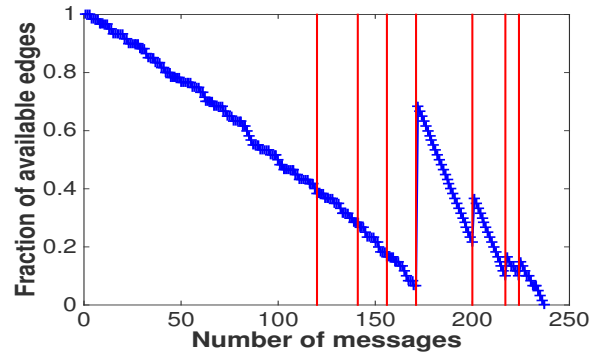
Figure 5: Temporal user targeting attacks on Ostra, (a) without attack edge churn, when the target has less edges than the number of attack edges, and (b) with attack edge churn, when the target has more edges than the number of attack edges. We observe that the target user is eventually unable to receive communication from other honest users.
