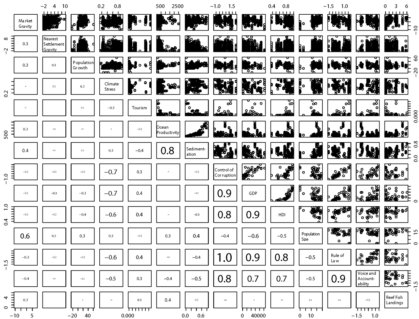
Extended Data Figure 2 | Correlation plot of candidate continuous covariates before accounting for collinearity (Extended Data Table 4).
