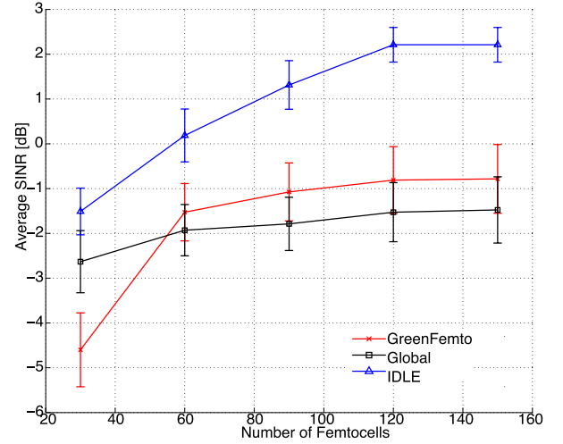
Fig. 9. Average SINR, 100 users, increasing femtocell scenario.
