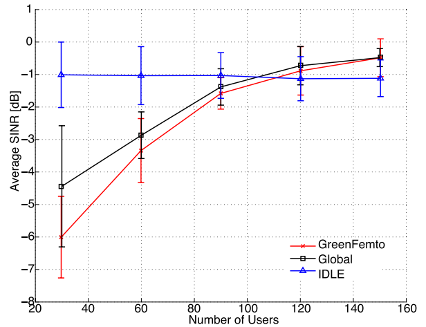
Fig. 5. Average SINR, 50 femtocells, increasing user scenario.
