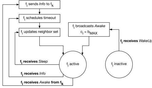
Fig. 3. Femtocell state diagram for message events.
