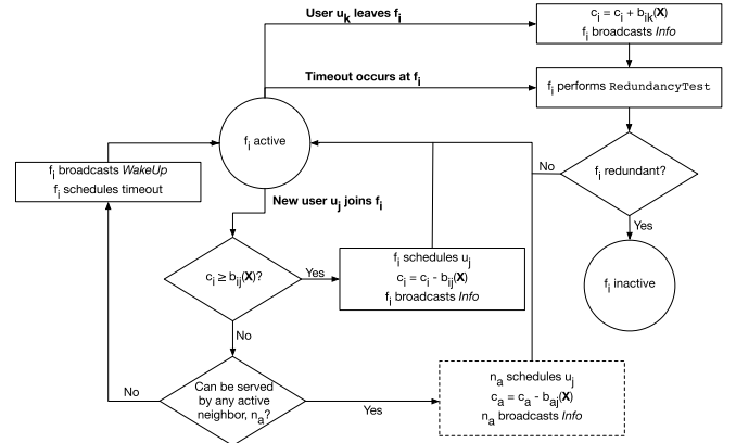
Fig. 2. Femtocell state diagram for user events.
