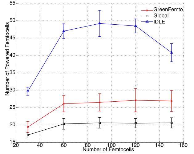
Fig. 8. Number of powered femtocells, 100 users, increasing femtocell scenario.
