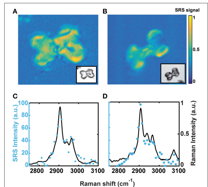
FIGURE 2 | Hyperspectral imaging of individual phytoliths from samples A and E shows OM is distributed unevenly throughout the silica matrix. Dark spots visible in optical microscopy do not contain OM and there are no obvious patterns in the OM distribution. (A, B) Show one end-member of the VCA for phytolith A and E hyperspectral imaging. Insert is the corresponding optical image. (C, D) are the Raman spectra in the CH region (solid line is average of all spectra, blue dots are specific SRS intensity measures).
