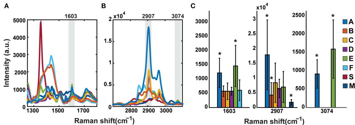
FIGURE 4 | Comparison of mean non-normalized signal intensities shows variability by sample treatment. Samples A, C, D, and E show common features both in the fingerprint region (A) and the CH stretching region (B). Sample M is less similar but retains some characteristics of the above. Samples B and F show a broad higher intensity set of peaks in the fingerprint region and lower intensities in the CH stretching region from the other samples. (C) is the statistical comparison of peaks 1603, 2907, and 3074 \text{cm}^{-1} . Sample A has the highest relative intensity at 2907 \text{cm}^{-1} . Asterisks denote statistical differences ( p < 0.05 ).
