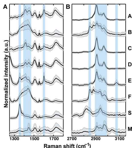
FIGURE 3 | Raman spectroscopy results for bilobate phytoliths from treatments A–F, and S, and trapezoidal phytoliths from M. Variability in peak locations and relative intensities, designated by vertical bars, indicate locations of Raman band disparities. Spectrum averages (heavy line) and variability (gray area, \pm 1 standard deviation) within each sample ( n = 30 ) in the fingerprint region ( A ) and the CH region ( B ) are shown. Samples B, F, S, and M exhibited the largest standard deviation from their average spectra.
