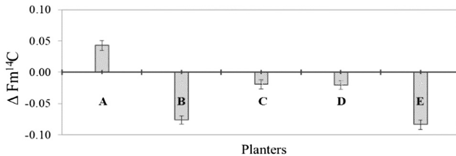
Fig. 4. Radiocarbon offsets between phytC and Sorghum bicolor plants grown under similar conditions, except that the soil amendments had different ^{14}\text{C} signatures. Phytoliths were extracted using a wet-digestion protocol (termed 1a in Reyerson et al. (2016) ). Offset values were correlated to the ^{14}\text{C} signatures of the amendments. The Planter A amendment was composed of rich bulk-complex organic C imprinted with ^{14}\text{C} post-bomb values (or \text{Fm}^{14}\text{C} signatures higher than present-day values), while the Planter E amendment received a solution of fossil organic C ( \text{Fm}^{14}\text{C} = 0 ; ^{14}\text{C} age close to 43 kyr BP). On the right, the positive and negative offsets are represented by arrows.
