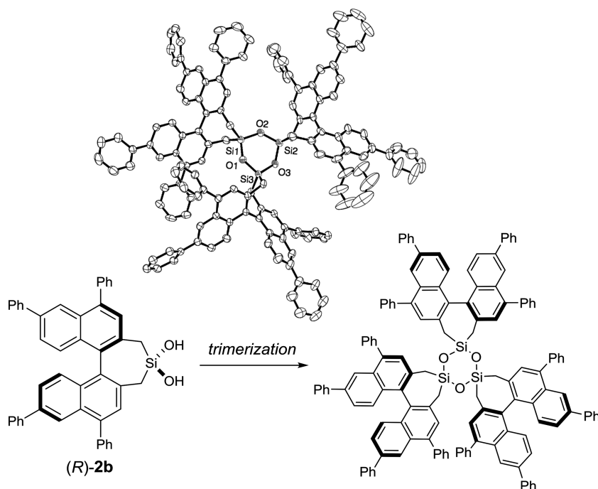
Figure 3. ORTEP representation of the trimer derived from ( R )- 2b . The anisotropic displacement parameters are drawn at the 50% probability level.
