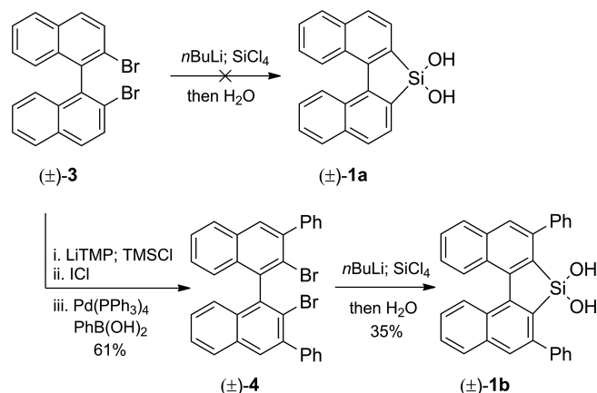
Scheme 2. Synthetic route to silanediol ( \pm )- 1b ; LiTMP = lithium tetramethylpiperide, TMSCl = trimethylsilyl chloride.
