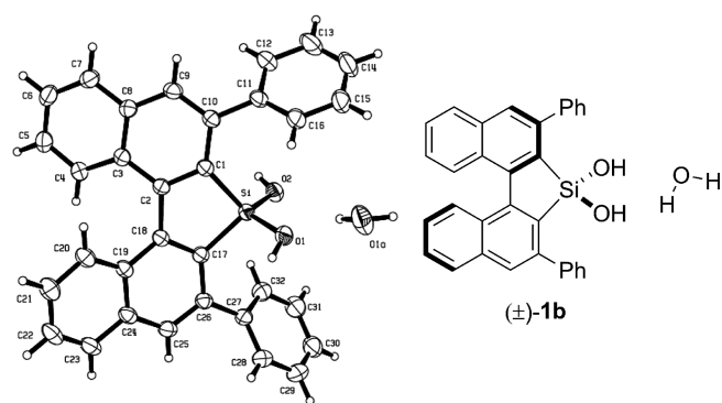
Figure 1. ORTEP representation of the H 2 O complex of ( \pm )- 1b . The anisotropic displacement parameters are drawn at the 50% probability level.
