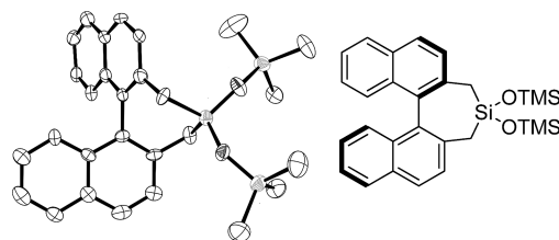
Figure 2. ORTEP representation of the bis-TMS derivative of ( R )- 2a . The anisotropic displacement parameters are drawn at the 50% probability level.
