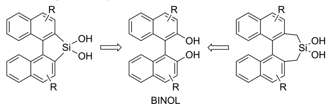
Scheme 1. BINOL-based silanediol catalyst designs.
