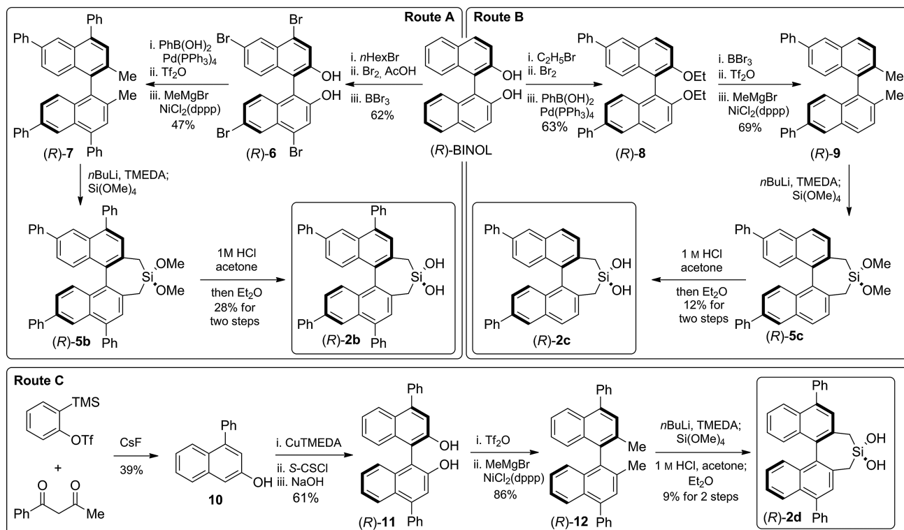
Scheme 4. Synthesis of the 4,4'- and 6,6'-substituted silanediols ( R )- 2b , ( R )- 2c , and ( R )- 2d .
