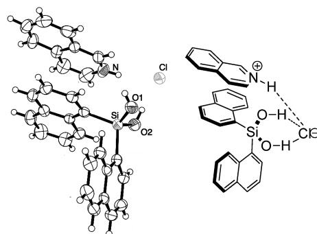
Figure 6. ORTEP representation of the ion pair between 14 and the HCl salt of isoquinoline. The anisotropic displacement parameters are drawn at the 50% probability level. [23]
