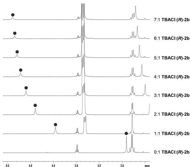
Figure 4. ^1H NMR binding titration of silanediol ( R )- 2b and nBu_4NCl in CDCl_3 .
