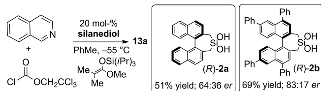
Scheme 5. Comparison of silanediol catalysts ( R )- 2a to ( R )- 2b under optimized reaction conditions.
