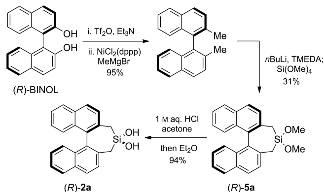
Scheme 3. Synthesis of unsubstituted silanediol ( R )- 2a .
