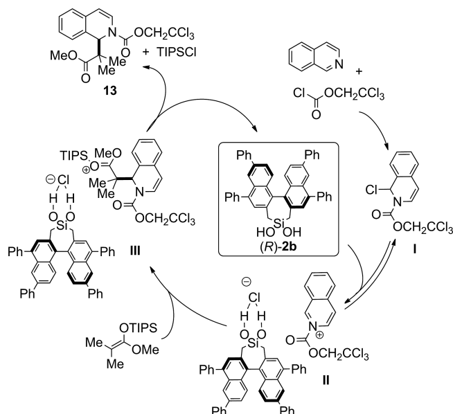
Scheme 6. Proposed reaction pathway for the silanediol-catalyzed N -acyl Mannich reaction of isoquinolines.
