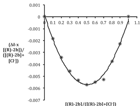
Figure 5. Job Plot analysis of ( R )- 2b and nBu_4NCl in CDCl_3 .
