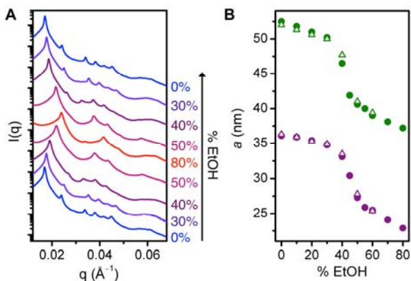
Figure 2. (A) SAXS data for BCC superlattices of 30 nm PAEs at different volume percentages of EtOH in H 2 O. (B) BCC unit cell length, a , for superlattices of 30 nm PAEs (green) and 15 nm PAEs (purple) at different volume percentages of EtOH in H 2 O. Solid and empty symbols correspond to values during contraction and
