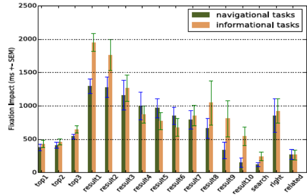
(b) SearchGazer
