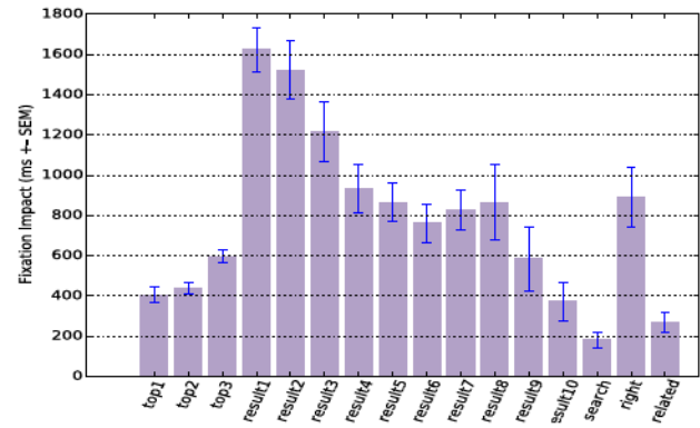
(b) SearchGazer
