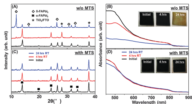
Fig. 1 Evolution of XRD patterns and UV-vis spectra of phase-pure \alpha\text{-FAPbI}_3 perovskite thin films before and after exposure to the ambient (RT, 45 \pm 5\% relative humidity): (A and B) without MTS (planar) and (C and D) with MTS. Insets in (B) and (D) are corresponding to optical photographs of the thin films.
