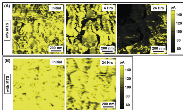
Fig. 2 Conductive AFM maps of \alpha -FAPbI 3 perovskite thin film as a function of ambient-exposure time: (A) without MTS (planar) and (B) with MTS.
