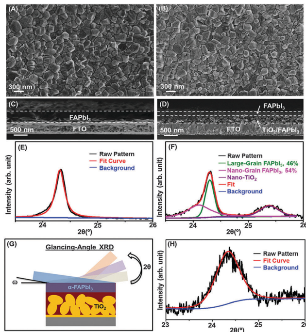
Fig. 3 Top-view and cross-sectional SEM images of \alpha -FAPbI 3 perovskite thin films: (A and C) without MTS (planar) and (B and D) with MTS. XRD patterns and fits of the \alpha -FAPbI 3 perovskite thin films: (E) without MTS (planar) and (F) with MTS. (G) Schematic illustration of glancing-angle XRD and (H) corresponding XRD pattern and fit of the \alpha -FAPbI 3 perovskite thin film with MTS.
