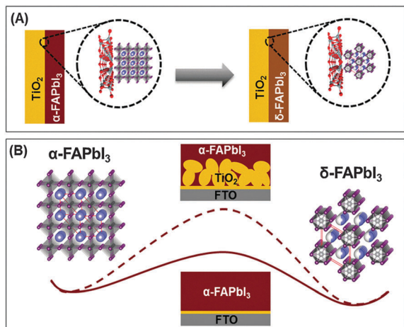
Fig. 4 Schematic illustrations: (A) highlighting the difference in the interface characteristics of \alpha -FAPbI 3 /TiO 2 and \delta -FAPbI 3 /TiO 2 interfaces and (B) depicting the increase of the energy barrier for the \alpha -FAPbI 3 \rightarrow \delta -FAPbI 3 transformation with an increase in the FAPbI 3 /TiO 2 interfacial area.
