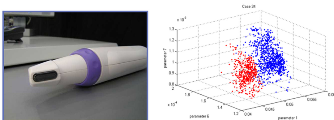
Figure 18. The photo (left) show the prototype intra-operative surgical probe for use during breast cancer surgery. The graph (right) show the classification of breast cancer data collected with the probe where tumour (red) is well separated from normal tissue (blue).
