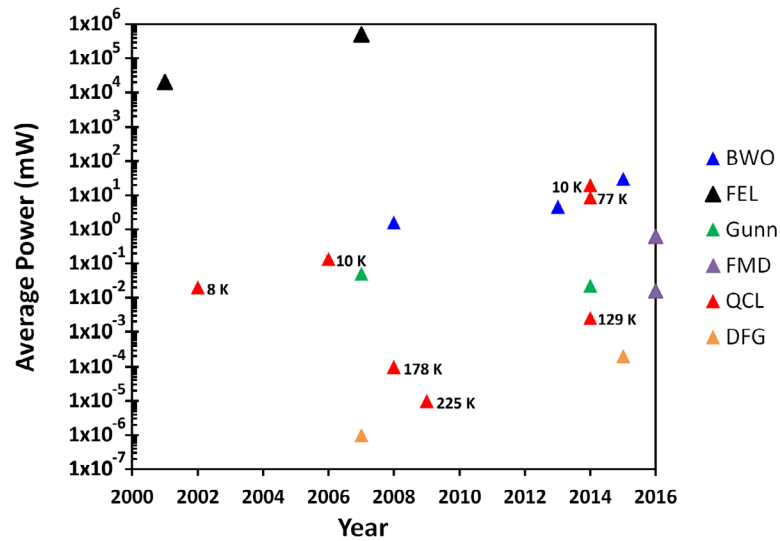
Figure 8. Progress of terahertz sources over recent years: BWO = backward wave oscillator ( \blacktriangle ), FEL = free electron laser ( \blacktriangle ), FMD = frequency multiplier devices ( \blacktriangle ), gunn diodes ( \blacktriangle ), QCL = quantum cascade laser (at 10 K unless otherwise stated) ( \blacktriangle ), DFG = difference frequency generation ( \blacktriangle ). All data are at room temperature unless otherwise stated.
