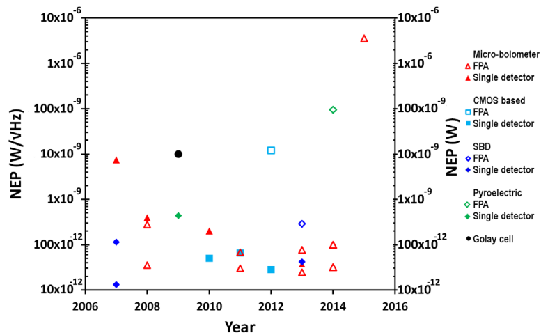
Figure 9. Progress of terahertz detectors over recent years: micro-bolometer based FPA ( \Delta ), micro-bolometer single detector ( \blacktriangle ), CMOS based FPA ( \square ), CMOS based single detector ( \blacksquare ), SBD FPA ( \diamond ), SBD single detector ( \blacklozenge ), pyroelectric FPA ( \diamond ), pyroelectric single detector ( \blacklozenge ) and Golay cell ( \bullet ). NEP for single detectors is on the left axis (closed symbols) and NEP for arrays is on the right axis (open symbols).
