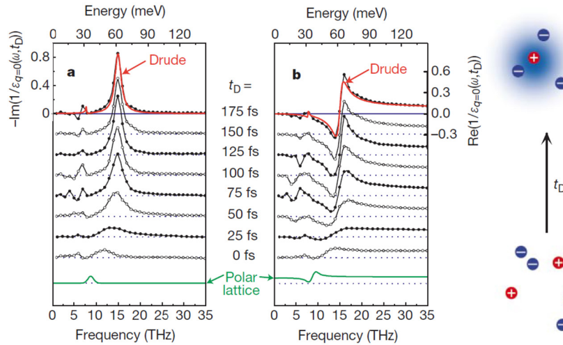
Figure 13. Imaginary (a) and real (b) parts of the inverse dielectric function of GaAs upon photoexcitation. It is seen that the transition from independent electrons and holes to an ensemble of screened quasiparticles occurs on a time scale of 10–100 fs. Reproduced with permission from [111], copyright 2001, Nature Publishing Group.
