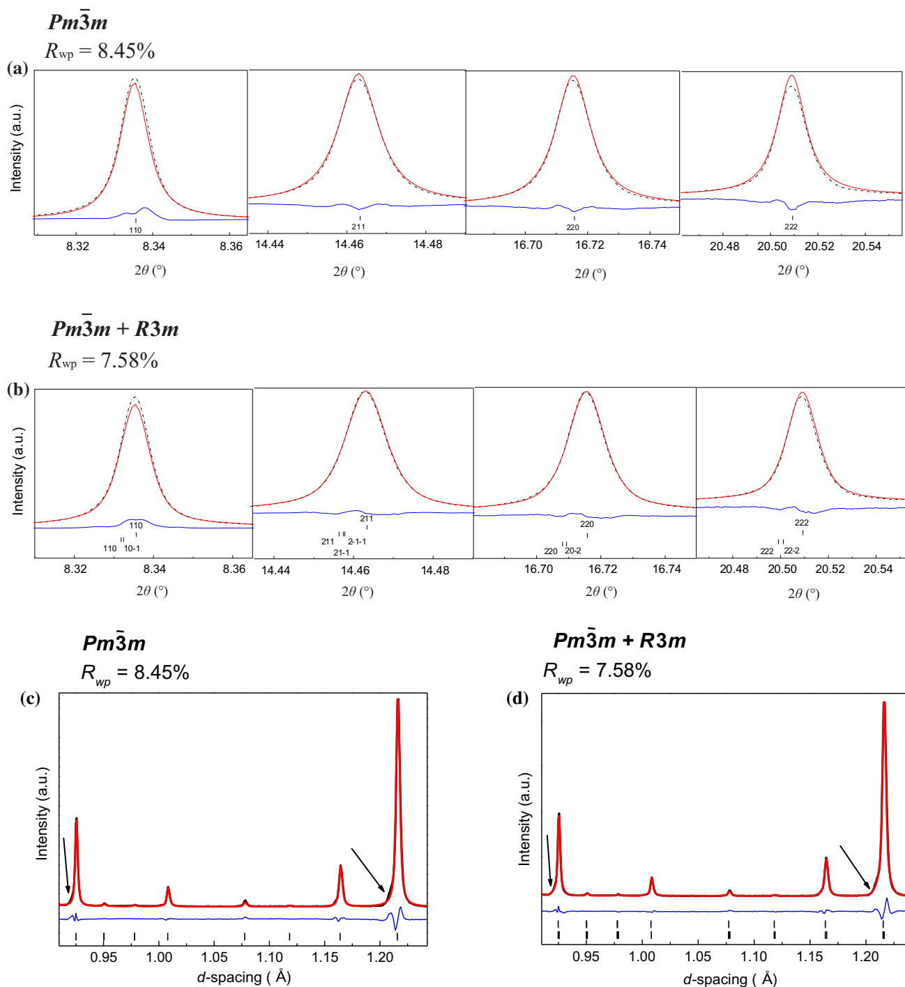
Fig. 3 The fits of selected reflections in Rietveld refinements of x = 0.12 using a–c single-phase Pm \bar{3} m and b–d multi-phase Pm \bar{3} m and R 3 m with the upper tic marks from Pm \bar{3} m and the lower tic marks from R 3 m . The SXRD data is on top and NPD
