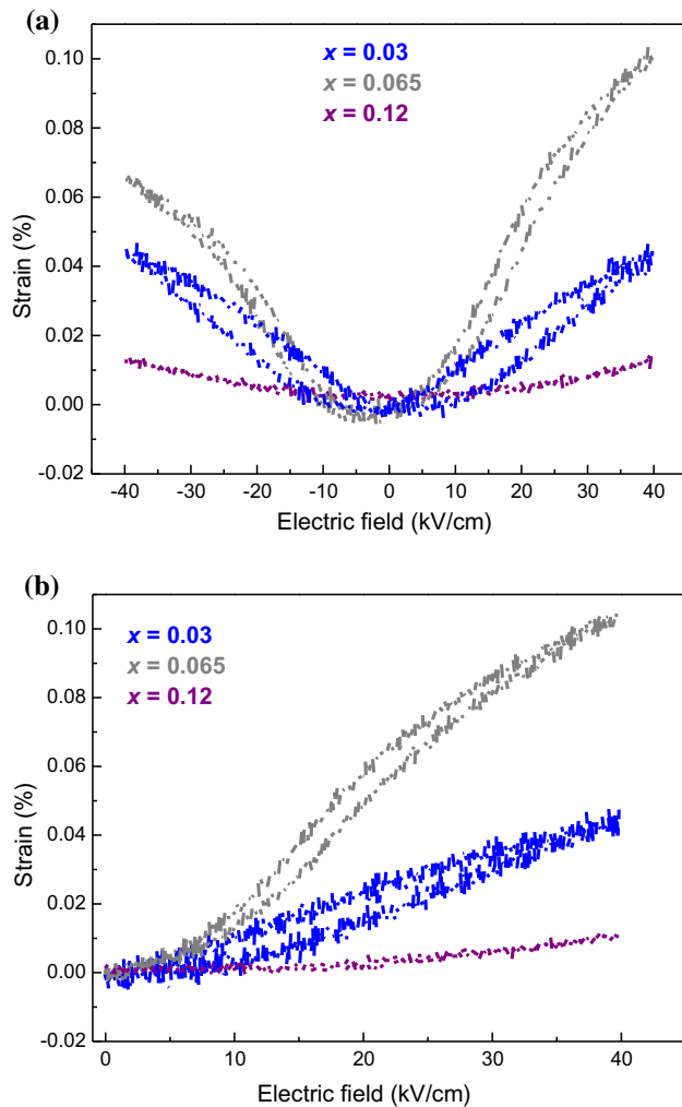
Fig. 7 For (1-x)\text{BT}-(x)\text{BI} ceramics room temperature: a bipolar and b monopolar strain-electric field measurements performed at 0.1 Hz for x = 0.03 (blue), x = 0.065 (gray) and x = 0.12 (purple).
