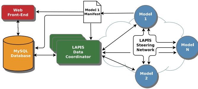
Fig. 3. LAPIS visualization system architecture.
