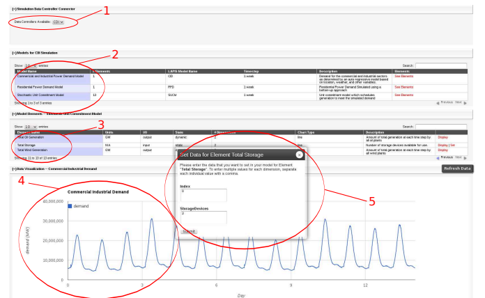
Fig. 4. Demonstration implementation of the ICS-EPP visualization model.
