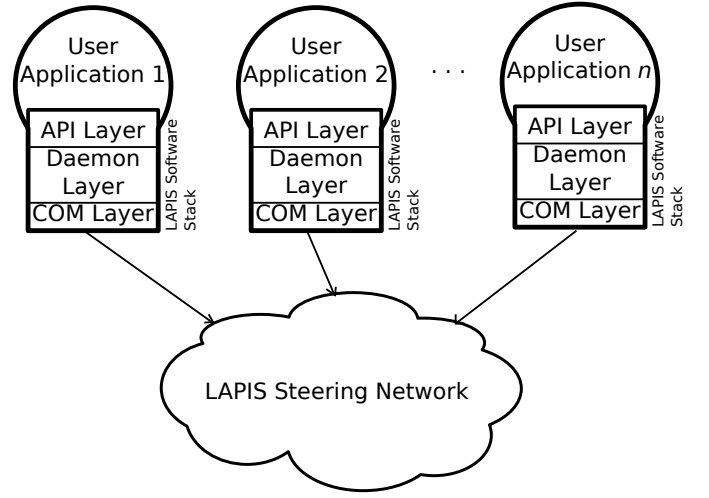
Fig. 5. The structure of the LAPIS system. LAPIS is as general purpose a steering system as possible. As such, the system makes no distinctions between nodes on the steering network.
