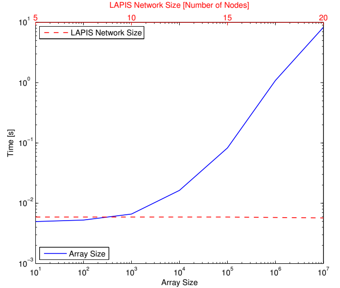
Fig. 6. Performance of the LAPIS system as a function of array and steering network size.
