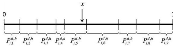
Fig. 4. Random simulation of state transition between two subsequent time periods [11].
