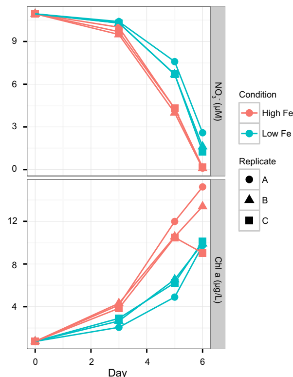
Fig. 1. Progression of Chlorophyll a (chl a) and nitrate ( \text{NO}_3^- ) concentrations during the course of the incubations. Nitrate concentrations at Day 0 are after the initial nutrient spike. High Fe incubations are in red, while Low Fe are in blue. Biological replicates are represented by different shapes. Note different scales in each subplot.
