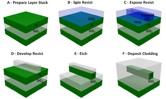
Fig. 3. Illustration of the fabrication process.
