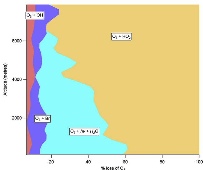
Fig. 5. The graph represents the contribution to O_3 loss in the FT and MBL from reaction with HO_2 (yellow), O^1D (blue), Br from inorganic halogens measured by the CIMS (purple) and OH (red). These values have been calculated from the steady state approximation explained in the SOM. (For interpretation of the references to colour in this figure legend, the reader is referred to the web version of this article.)
