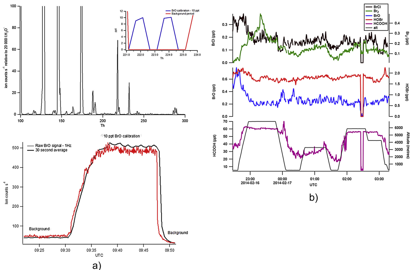
Fig. 1. a. BrO time series and mas scan during a calibration and background period. The standard deviations are reported for both 1 Hz and 30 s averaged data. b. Time series of in flight data utilising the nylon scrubber as a background technique for formic acid and the inorganic halogens.
