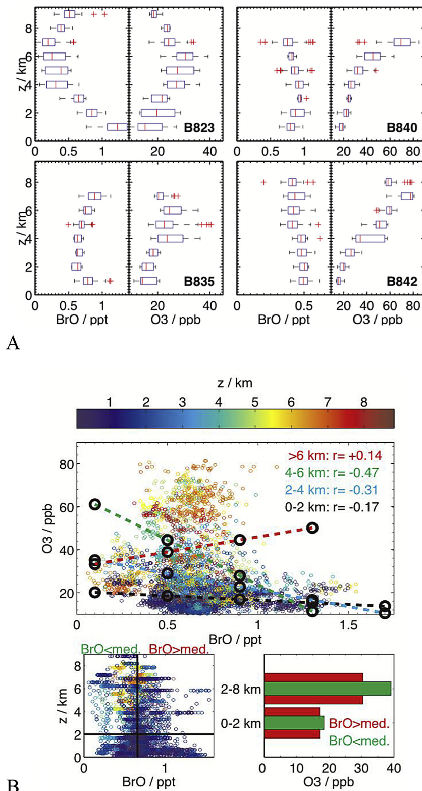
Fig. 3. Figure A shows altitude profile box plots of BrO and O 3 for 4 flights. The median, mean, 25th, 75th, 5th and 95th quartile ranges are indicated. Graph B shows a correlation plot of ozone and BrO split into 4 altitude bins (red > 6 km, green 4–6 km, blue 2–4 km, black 0–2 km) and also a bar chart of binned BrO data by altitude split into BrO concentrations above the 50th percentile (red) and below the 50th percentile (green). (For interpretation of the references to colour in this figure legend, the reader is referred to the web version of this article.)
