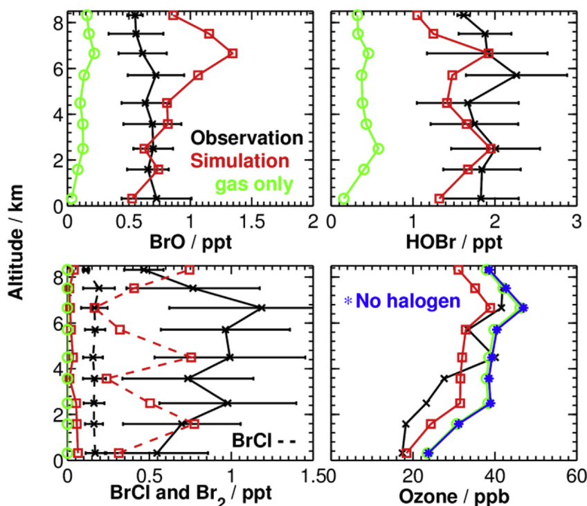
Fig. 4. Altitude profile box plot of the measured (CIMS) and modelled (GEOS-Chem) concentration of \text{BrO} (upper left), \text{HOBr} (upper right), \text{BrCl} (lower left, dashed), \text{Br}_2 (lower left, full), and ozone (lower right) throughout the campaign for 16 flights. Black lines represent the measurements. The red line is output from our GEOS-Chem simulation. The green curve is model output from a simulation without multiphase halogen chemistry (no oxidation of \text{Br}^- and \text{Cl}^- and no halogen release from SSA). The cyan curve shows simulated ozone when halogen chemistry is not included. The horizontal bars on the observed data lines correspond to the maximum and minimal values in the data set. (For interpretation of the references to colour in this figure legend, the reader is referred to the web version of this article.)
