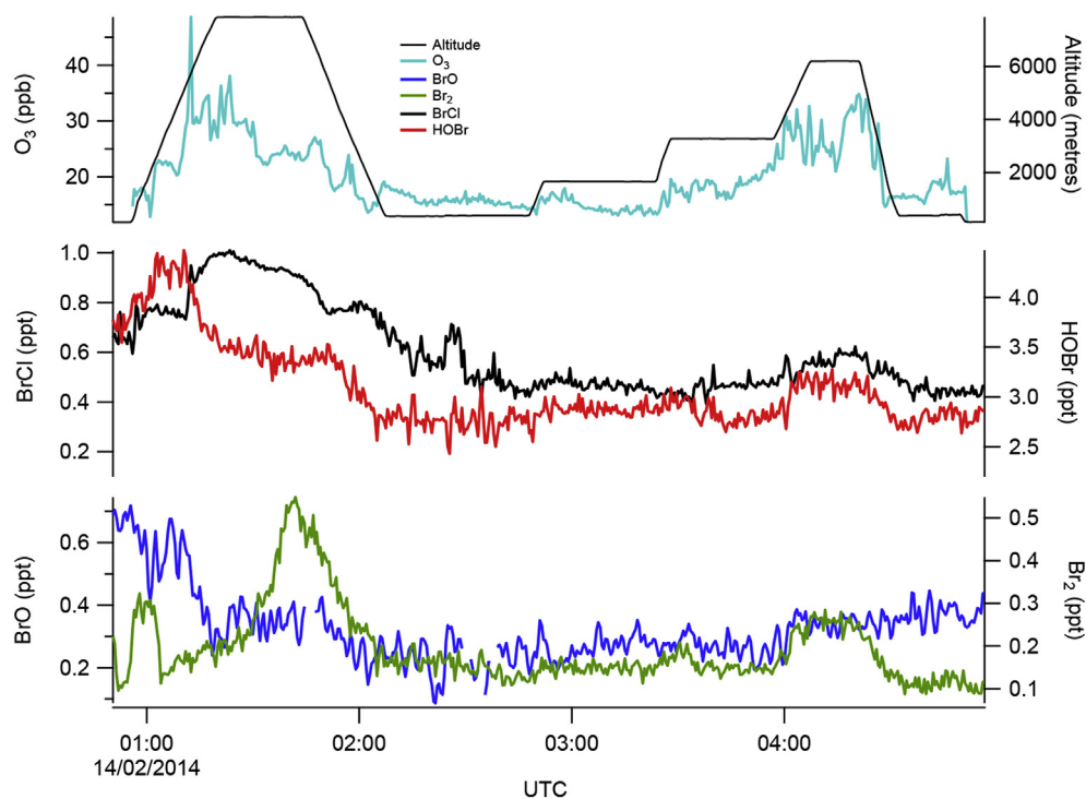
Fig. 2. A time series during flight B841 (14/02/14) of BrO (blue), Br 2 (green), HOBr (red) and BrCl (black) 30 s averaged concentrations from the CIMS and O 3 (light blue). The aircraft altitude (black) is also displayed. (For interpretation of the references to colour in this figure legend, the reader is referred to the web version of this article.)
