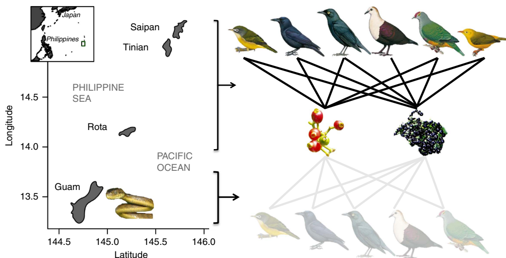
Figure 1 | Study site. Guam, the southernmost island in the Mariana Islands, is home to the invasive brown treesnake and thus virtually all forested lands are bird-free, whereas the nearby islands of Saipan, Tinian and Rota are snake-free, and have relatively healthy bird communities. On islands with birds, the primary frugivores (from left to right) for two tree species whose fruits are depicted in the middle, Psychotria mariana (left) and Premna serratifolia (right), include the bridled white-eye ( Zosterops conspicillatus ), and Rota bridled white-eye ( Zosterops rotensis ; both Zosterops species represented by the bridled white eye in the figure), Mariana crow ( Corvus kubaryi ), Micronesian starling ( Aplonis opaca ), white-throated ground dove ( Gallicolumba xanthonura ; Premna only), Mariana fruit dove ( Ptilinopus roseicapilla ) and golden white-eye ( Cleptornis marchei ). As a result of the snake, Psychotria mariana and Premna serratifolia on Guam have functionally lost all of their seed dispersing partners (note that the Rota bridled white-eye and the golden white-eye were not on Guam before the snake introduction). Latitude and longitude are in degrees north and east, respectively. Snake photograph and bird illustrations 54–59 used with permission.
