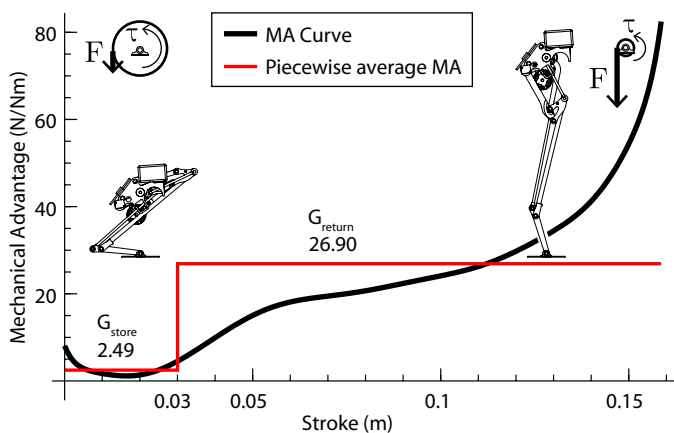
Fig. 5. MA as a function of leg extension. Average values of G_{\text{store}} and G_{\text{return}} for energy storage and return phases are shown. Cartoons show the leg mechanism fully crouched and fully extended.
