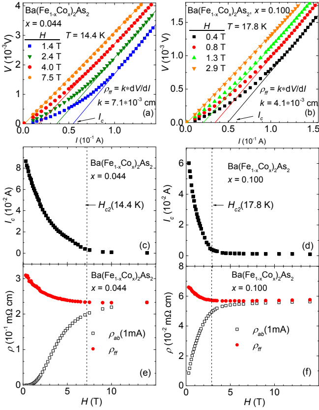
FIG. 4. Current-voltage I - V curves measured at different magnetic field H values in the mixed state of \text{Ba}(\text{Fe}_{1-x}\text{Co}_x)_2\text{As}_2 with (a) x = 0.044 at a temperature T of 14.4 K and (b) x = 0.100 at T = 17.8 K. Plots of the critical current I_c vs H for (c) x = 0.044 and (d) x = 0.100 . (e) H dependence of the flux-flow resistivity \rho_{ff} (filled circles) and the resistivity \rho_{ab} measured with a constant current of 1 mA applied parallel with the ab plane of the single crystals (open squares) for the (e) the x = 0.044 and (f) x = 0.100 samples.
