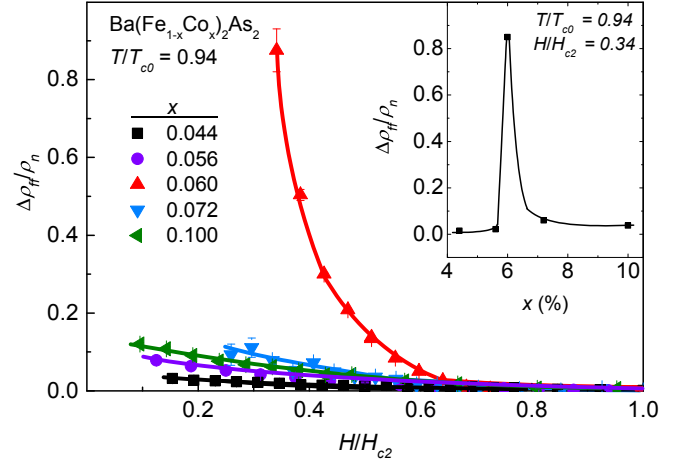
FIG. 6. Normalized flux-flow resistivity \Delta\rho_{ff}/\rho_n \equiv \rho_{ff}/\rho_n - 1 as a function of reduced magnetic field H/H_{c2} measured at the same reduced temperature T/T_c = 0.94 for all Co doping values x . Inset: \Delta\rho_{ff}/\rho_n vs x measured at T/T_c = 0.94 and H/H_{c2} = 0.34 for all the single crystals studied.
