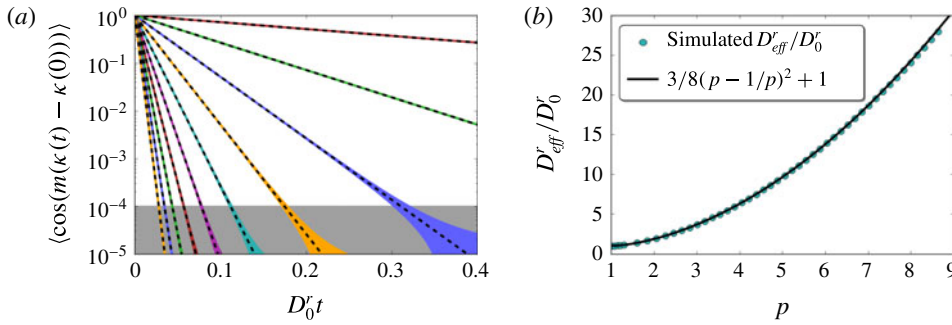
FIGURE 2. (Colour online) Rotational diffusion under continuous shear in the stretched \kappa -space. (a) Semi-log plot of the correlations \langle \cos(m\Delta\kappa) \rangle versus time for an aspect ratio p \approx 2.83 and Pe = 10^4 . The black dotted lines correspond to diffusive correlations with the diffusion constant from (2.15); the coloured lines correspond to the simulated correlations. There is excellent agreement with no adjustable parameters. At long times, higher-order corrections in 1/Pe are visible as the broadening into bands when the correlations decrease below \approx 10^{-4} (grey shaded region). (b) The diffusion constant D_{eff}^r , extracted from simulated m = 1 correlations, plotted versus aspect ratio (cyan circles), alongside the prediction from (2.15) (black line).
