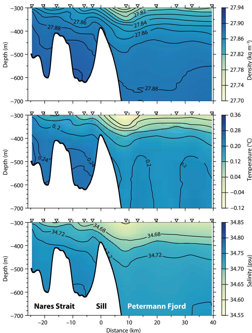
FIGURE 5. Section for depths below 300 m from Nares Strait to the terminus of Petermann Gletscher showing the density anomaly in \text{kg m}^{-3} (top panel), potential temperature in ^\circ\text{C} (middle panel), and salinity in psu (bottom panel) as observed on August 10–11, 2012.
