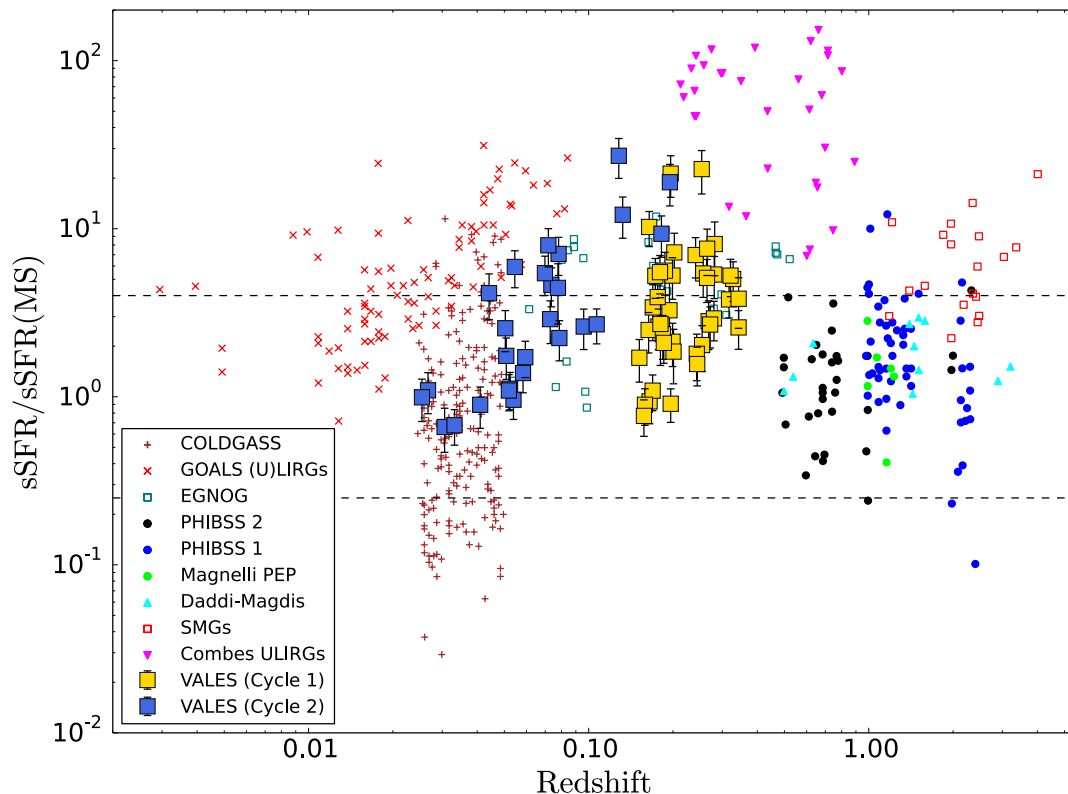
Figure 1. The figure shows the specific Star Formation Rate (sSFR, defined as \text{sSFR} = \text{SFR}/M_* ), normalised to the one estimated for the ‘main sequence’ (Elbaz et al. 2011; Whitaker et al. 2012) as a function of redshift for different samples of galaxies detected in CO. We use the parametrisation of the ‘main sequence’ made by Genzel et al. (2015) as \log[\text{sSFR}(\text{MS}, z, M_*)] = -1.12 + 1.14z - 0.19z^2 - (0.3 + 0.13z) \times (\log M_* - 10.5) \text{ Gyr}^{-1} , where dashed black lines denote 0.6 dex off this equation for star-forming galaxies. Our data is presented in filled squares with error bars taken from our ALMA Cycle-1 (yellow) and Cycle-2 (royal blue) campaigns. We estimate the SFR using L_{\text{IR}}(8 - 1000 \mu\text{m}) extracted from the H -ATLAS data, stellar masses using MAGPHYS fits (see § 2.4.3) – both using the same IMF, and redshifts taken from the GAMA survey. Dark red crosses are nearby galaxies (Saintonge et al. 2011), red crosses are (U)LIRGs (Howell et al. 2010), light blue unfilled squares are z = 0.05 - 0.5 normal galaxies (Bauermeister et al. 2013), pink inverted triangles are ULIRGs at intermediate redshifts (Combes et al. 2011, 2013), blue dots are ‘main sequence’ galaxies at z = 1 - 1.5 and 2 - 2.5 (Tacconi et al. 2010, 2013), black dots are ‘main sequence’ galaxies at z = 0.5 - 1 and z \sim 2 (Combes & the PHIBSS collaboration 2015), light blue triangles are ‘main sequence’ galaxies at high- z (Magnelli et al. 2012), light green dots are ‘main sequence’ galaxies at z = 0.5 - 3.2 (Daddi et al. 2010a; Magdis et al. 2012) and red unfilled squares are sub-millimetre galaxies at z = 1.2 - 3.4 (Greve et al. 2005; Tacconi et al. 2006, 2008; Bothwell et al. 2013). Figure adapted from Genzel et al. (2015).
