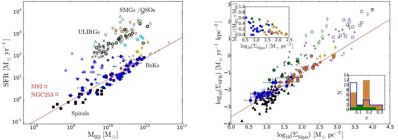
Figure 6. Left: The SFR versus M_{H_2} for our galaxies compared to previous works taken from the literature (assuming a Chabrier’s IMF but considering the same \alpha_{CO} used in the original works). We show our spectrally detected (blue circles), spectrally undetected but measured with low signal to noise in collapsed cubes (stars), and undetected (blue arrows) CO galaxies (see § 2.4 for details). Blue filled symbols are B- and D-dominated galaxies, while blue unfilled symbols are M-dominated galaxies. Figure contains BzK galaxies (Daddi et al. 2010a; gold diamonds), z \sim 0.5 disk galaxies (Salmi et al. 2012; red filled triangles), z = 1-2.3 normal galaxies (Tacconi et al. 2010; brown crosses), SMGs (Greve et al. 2005; Frayer et al. 2008; Daddi et al. 2009a,b; red down triangles, Ivion et al. 2011; unfilled cyan hexagons), QSOs (Riechers et al. 2006; green triangles), local ULIRGs (Solomon et al. 1997; black crosses), strongly lensed high-redshift dusty star forming galaxies (Aravena et al. 2016; black unfilled circles), and local spirals (Leroy et al. 2009; black filled squares; Wilson et al. 2009; black filled triangles). M82 and NGC 253 are also shown (Weiß et al. 2001; Houghton et al. 1997; Kaneda et al. 2009). The solid red line is the best fit for the B- and D-dominated galaxies presented in this work (see Eqn. 4). Right: The SFR surface density as a function of the gas mass (atomic and molecular) surface density for the 21 detected sources that can be spatially resolved in CO (blue circles; see § 3.3), 23 detected B- and D-dominated which are unresolved in CO but resolved in R -band (brown circles), and M-dominated unresolved in CO galaxies (green circles). Filled triangles are (U)LIRGs and spiral galaxies from the sample of Kennicutt (1998), brown crosses are z = 1-2.3 normal galaxies (Tacconi et al. 2010). The empty blue squares and light green diamonds are SMGs from Bouché et al. (2007) and Bothwell et al. (2009), respectively. The red line is the best linear fit to all of our B- and D-dominated galaxies (see Eqn. 6). The inset figures at the upper left and bottom right corners are: (1) the relative contribution estimated by M_{HI} following Eqn. 5 to the total gas mass ( M_{H_2} + M_{HI} ) versus \Sigma_{Mgas} . This figure demonstrates the decreasing effect that M_{HI} has at \Sigma_{Mgas} > 10 M_{\odot} \text{ pc}^{-2} ; (2) the redshift distribution of our VALES galaxies (blue, yellow and green circles), clearly showing that most of the spatially unresolved galaxies are the ones which are more distant.
