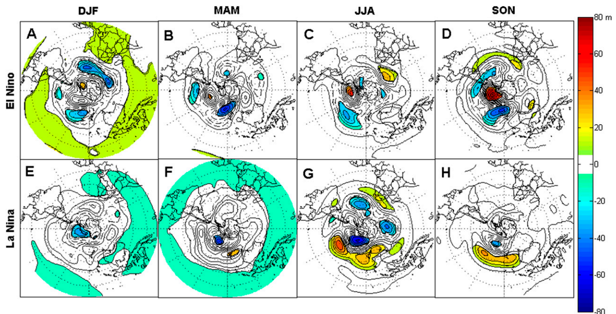
FIG. 3. As in Fig. 2, but for 500-hPa geopotential heights.
