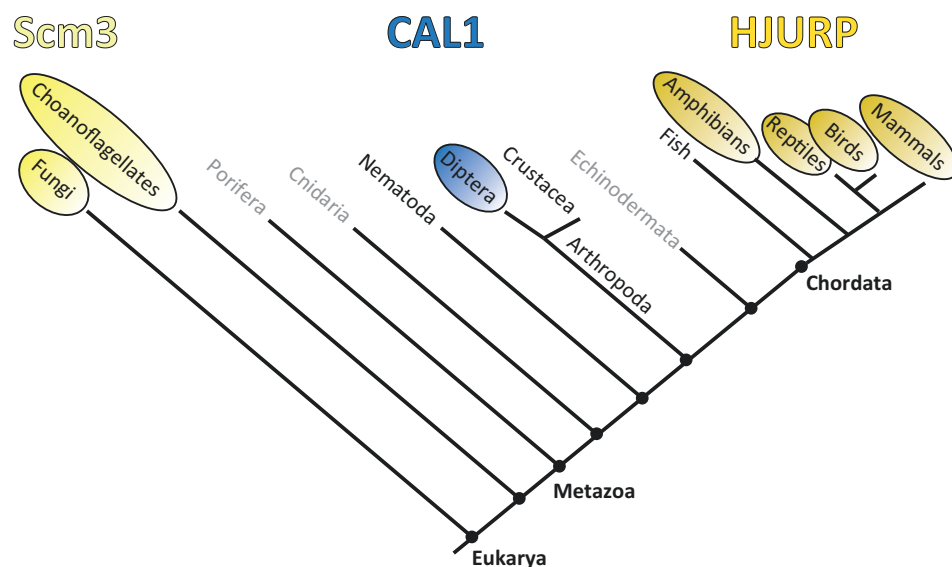
Figure 1. Phylogenetic Relationships of Known CENP-A Assembly Factors. Yellow circles represent taxa with Scm3/HJURP homologs. Blue circles indicate the birth of a novel CENP-A chaperone. The taxa lacking circles have no known CENP-A chaperone, while taxa in gray have yet to be examined.
