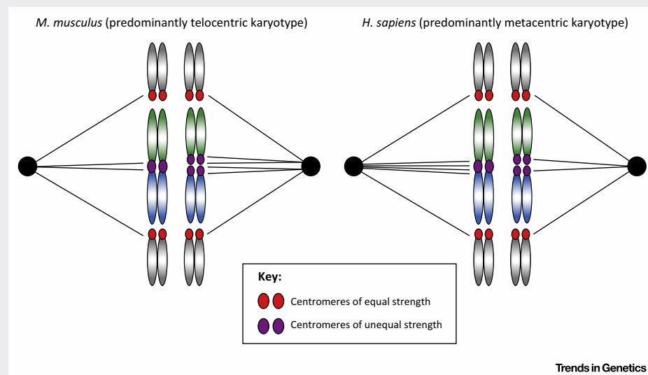
Figure 1. The Formation of Robertsonian Fusions Results in an Asymmetric Bivalent Composed of the Rb Chromosome Paired with Its Two Unfused Counterparts. Which centromere is stronger seems to depend on the background karyotype of the species. The two telocentric centromeres would be stronger in a mouse species with a predominantly telocentric karyotype (left), while the Rb fusion would be stronger when the karyotype is predominantly metacentric, such as in humans (right).
