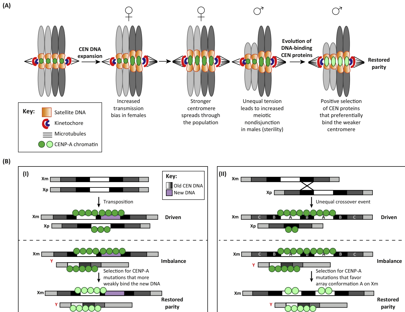
Figure 3. (A) The two-step model for centromere drive [109]. In the first step, satellite expansion results in a transmission bias during female meiosis, but nondisjunction during male meiosis, preventing the expansion from reaching fixation. In the second step, suppressor mutations in CENP-A or other centromeric (CEN) DNA binding proteins are selected for to restore meiotic parity. These CENP-A alleles either increase microtubule binding to the weaker centromere (as shown), or reduce microtubule binding to the driven centromere (not shown). Either types of mechanisms are proposed to restore meiotic parity. (B) Possible models of how CENP-A alleles with altered DNA binding preferences could restore meiotic parity according to centromere drive [83]. (BI) Centromere expansion occurs via the transposition of mobile DNA elements. Centromere balance is restored by the selection of CENP-A alleles that have increased preference for binding to the original centromeric sequences. (BII) Centromere expansion occurs after an unequal crossover event during meiosis I. The expansion does not contain new DNA sequences, but may have altered periodicity of monomers due to the insertion, allowing for CENP-A mutations that preferentially interact with certain DNA conformations to be selected for. CENP-A, centromere protein A.
