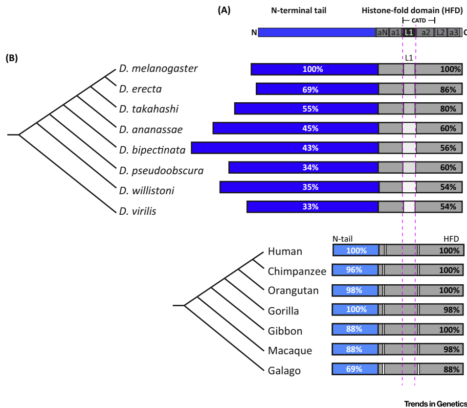
Figure 2. CENP-A Protein Domains and Conservation. (A) Diagram showing the primary structure of CENP-A. The N-terminal tail is shown in blue, the histone-fold domain (HFD) is shown in gray. The CATD and L1 are indicated (see text for details). (B) Schematic of CENP-A orthologs from several Drosophila (top) and primate (bottom) species. Rapidly evolving residues in the C-terminal HFD are indicated by lighter boxes. Percentages indicate the identity of the N-terminal tails or HFD to Drosophila melanogaster or Homo sapiens . Note that L1 displays slight size variation.
