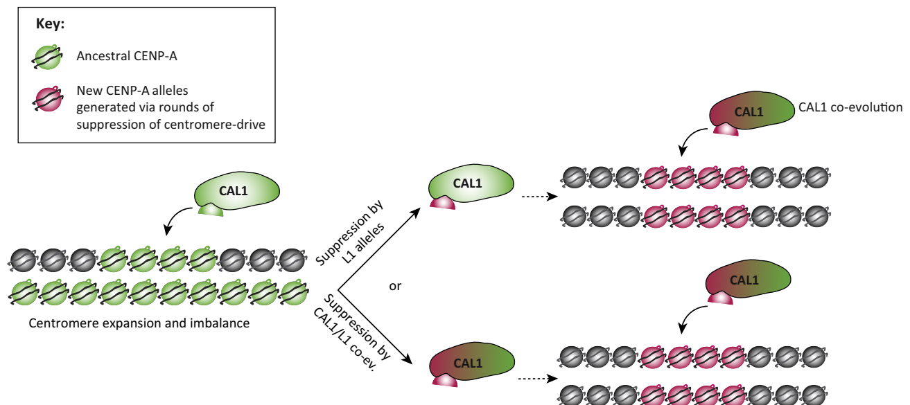
Figure 5. Model for Centromere Evolution in Drosophila . Centromere expansion in the ancestral species results in the selection of new CENP-A/CAL1 pairs that suppress drive. It is possible that new CENP-A L1 alleles themselves suppress drive through preferential interaction with DNA, and CAL1 subsequently co-evolves to maintain centromere identity (top). Alternatively, selection of L1 alleles might occur via the interaction with CAL1, resulting in changes in levels of CENP-A deposited [111] (bottom). CENP-A, centromere protein A.
