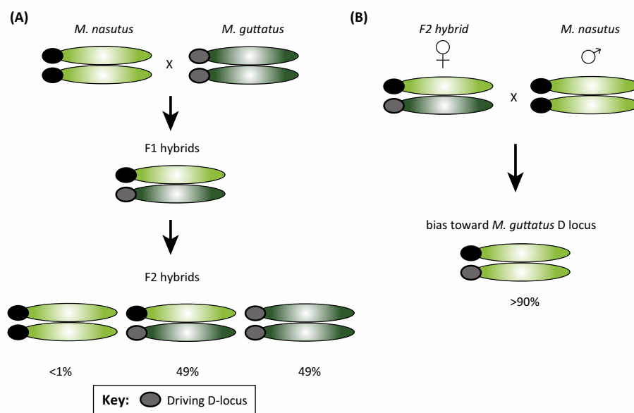
Figure I. Preferential Segregation of the D Locus in Monkeyflowers. (A) Mimulus nasutus (maternal; dd ) × Mimulus guttatus (paternal; DD ) F2 hybrids were used to determine that inheritance of the D locus (marked by the oval) and other nearby loci deviated from the expected Mendelian segregation ratios (0:2:2 rather than the Mendelian 1:2:1 dd : Dd : DD ). (B) By repeated backcrossing of F2 hybrids to the M. nasutus parental line ( dd ; paternal), it was discovered that despite most of the genome being homozygous for M. nasutus alleles, the D locus remained over 90% heterozygous. This suggested that the D locus from M. guttatus was being selected for. Adapted from [134].
