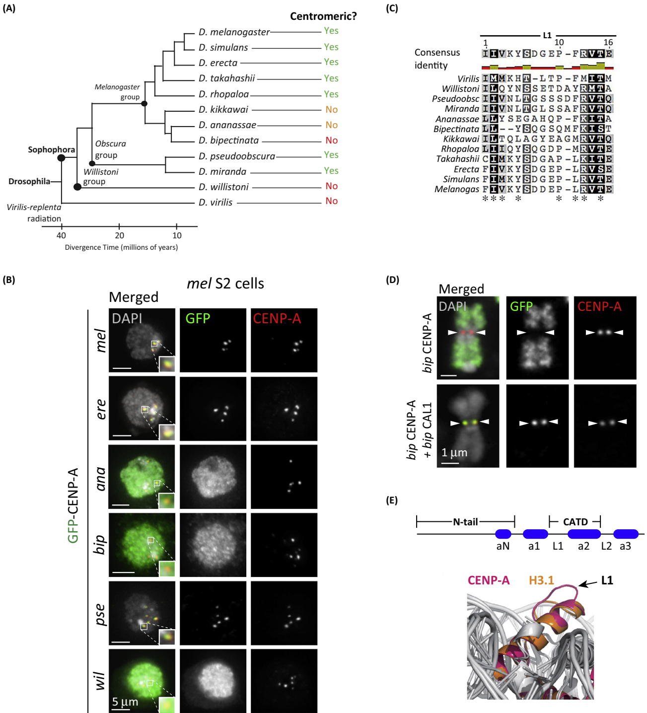
Figure 4. Incompatibility between Divergent CENP-A and the Assembly Factor CAL1 in Drosophila . (A) Phylogenetic tree of the Drosophila species with indicated divergence time and phylogenetic grouping based on FlyBase [126]. The localization of divergent CENP-A orthologs in Drosophila melanogaster cells is indicated to the right. Green indicates complete centromeric localization, orange partial centromeric localization, red non-centromeric localization. (B) Immunofluorescence images of interphase D. melanogaster S2 cells transiently expressing GFP-tagged CENP-A orthologs from mel ( D. melanogaster ), ere ( Drosophila erecta ), ana ( Drosophila ananassae ), bip ( Drosophila bipectinata ), pse ( Drosophila pseudoobscura ), and wil ( Drosophila willistoni ). DAPI is shown in gray, GFP in green, and mel CENP-A in red. Zoomed insets show individual centromeres with merged colors. From [113]. (C) BLOSUM80 alignment of L1 from select species. Shading indicates (Figure legend continued on the bottom of the next page.)
