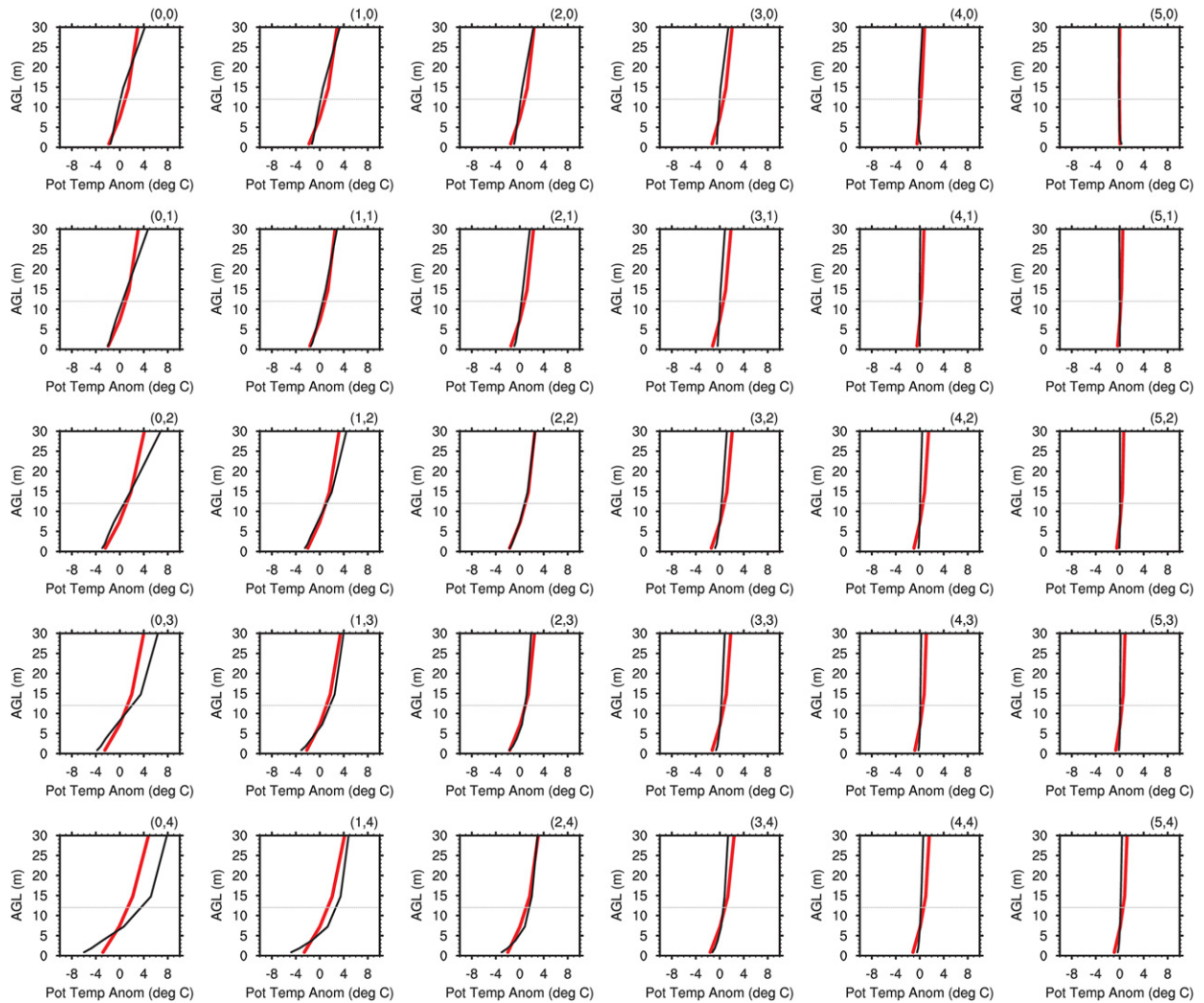
FIG. 6. The 30 SOM patterns average potential temperature anomaly profiles of Tall Tower observations (black line) and AMPS forecasts (red line).
