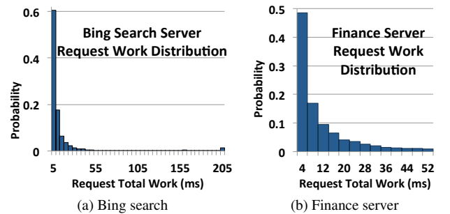
Figure 1: Work distribution of two interactive services: Bing search server (Kim et al. 2015a) and an option pricing finance server (Ren et al. 2013). Note that in Bing search server the probabilities of requests with work between 55ms to 200 are small but larger than zero and total probability of these requests is around 3.5%.
