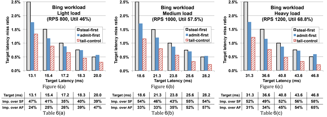
Figure 6: Results for the Bing workload with three different load settings and Poisson arrival. The x-axis shows different target latencies from shorter to longer from left to right. The y-axis shows the target latency miss ratio. The table below each figure shows tail-control's relative improvement over steal-first and admit-first for a given latency.
