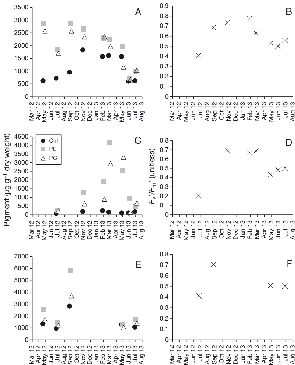
Fig. 3. Year-long pigment and photosynthetic yield data for all 3 study sites: (A,B) the Fountain; (C,D) El Cajon; (E,F) Middle Island Sinkhole. (A,C,E) show pigment data (Chl: chlorophyll; PE: phycoerythrin; PC: phycocyanin). (B,D,F) shows photosynthetic yield ( F_v'/F_m' ). Data points are slightly offset due to overlapping points. Note that the scale for pigment concentration is different for each site, while yield is constant
