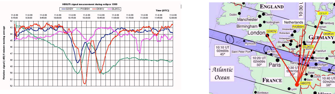
Figure 3. Relative signal strength from HBG Switzerland at 75 kHz during 1999 solar eclipse. https://misan.home.xs4all.nl/eclipse.htm
