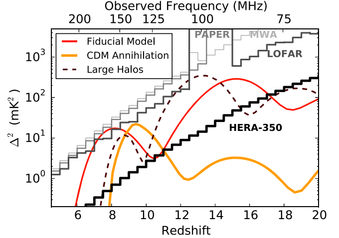
Figure 4. 1\sigma thermal noise errors on \Delta^2(k) , the 21 cm power spectrum, at k = 0.2 \, h \, \text{Mpc}^{-1} (the dominant error at that k ) with 1080 hr of integration (black) compared with various heating and reionization models (colored). Sensitivity analysis is per Table 1 and the associated text.
