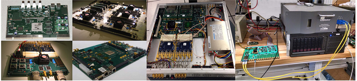
Figure 22. Six generations of CASPER digital signal processing (left to right) culminating in the SNAP board (right, along with the long-haul fiber-link test setup). By preserving its design tools, signal processing libraries, and interface code between hardware generations, CASPER hardware and a modular architecture have enabled the PAPER correlator to be easily upgraded for HERA (Parsons et al. 2006, 2008).
