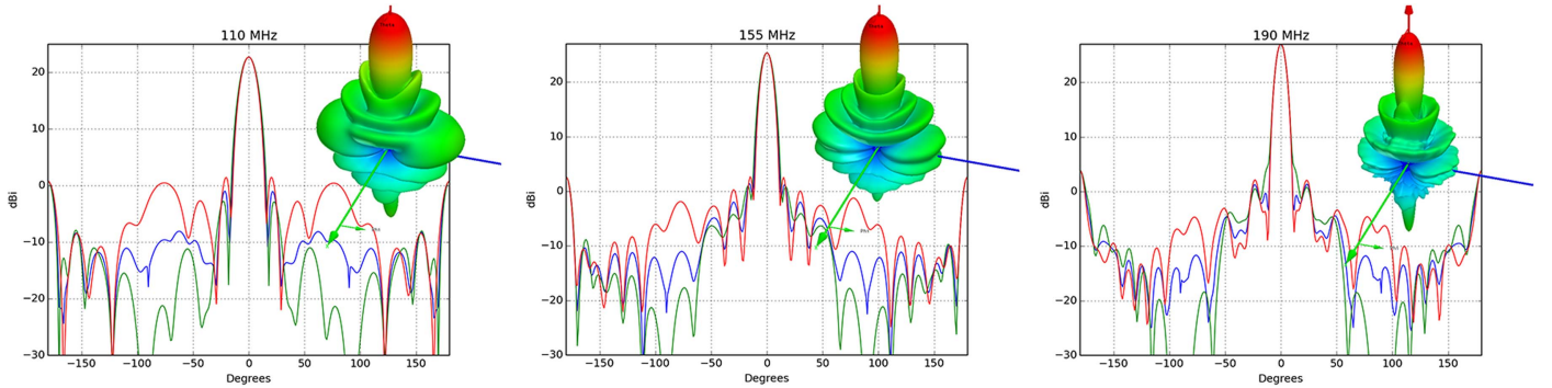
Figure 19. Antenna patterns at 110, 155 and 190 MHz calculated with HFSS and the adopted design. Red curves are E-plane, green are H-plane at blue at 45°. Inset is the full 3D pattern.
