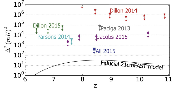
Figure 9. Current best published 2\sigma upper limits on the 21 cm power spectrum, \Delta^2(k) , compared to a 21 cm FAST-generated model at k = 0.2 \text{ h Mpc}^{-1} . Analysis is still underway on PAPER and MWA observations that approach their projected full sensitivities; HERA can deliver sub- \text{mK}^2 sensitivities.
