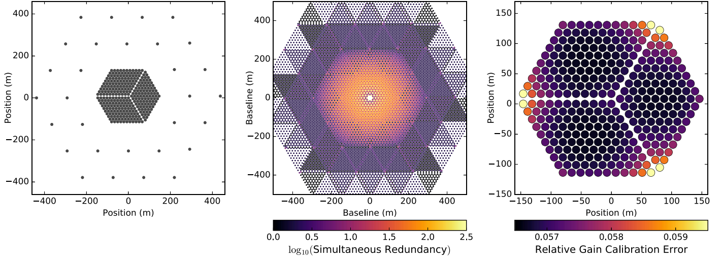
Figure 21. HERA’s elements are divided between a 320-element, hexagonally packed core and 30 outriggers (left). This produces instantaneous uv coverage at triple the element packing out to 250\lambda at 150 MHz, suppressing grating lobes in the synthesized beam (middle). All 350 elements can be redundantly calibrated using the Liu et al. (2010) technique, yielding calibration errors that are a small fraction of the residual noise per antenna (right). See Dillon & Parsons (2016) for discussion. (A color version of this figure is available in the online journal.)
