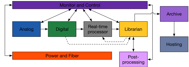
Figure 23. High-level architecture.
