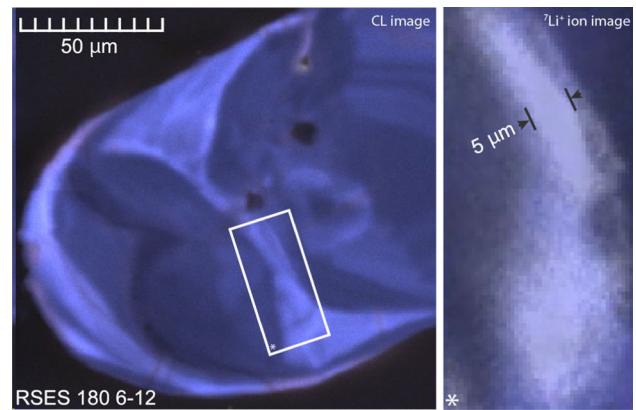
Fig. 9 Cathodoluminescence image of Jack Hills zircon RSES 180 6-12 showing complex internal zoning (left) with direct ion image of ^7\text{Li}^+ (right). The strong correlation of Li with the narrow zone separating two regions of igneous character likely limits post-formation Li diffusion to length scales less than ~5 microns and thus to subsequent peak heating temperatures not exceeding 500 °C for ca. million-year timescales. This example reasonably constrains the discovery location of the Jack Hills Hadean zircons to having never reached amphibolite facies conditions or the Curie temperature of magnetite
