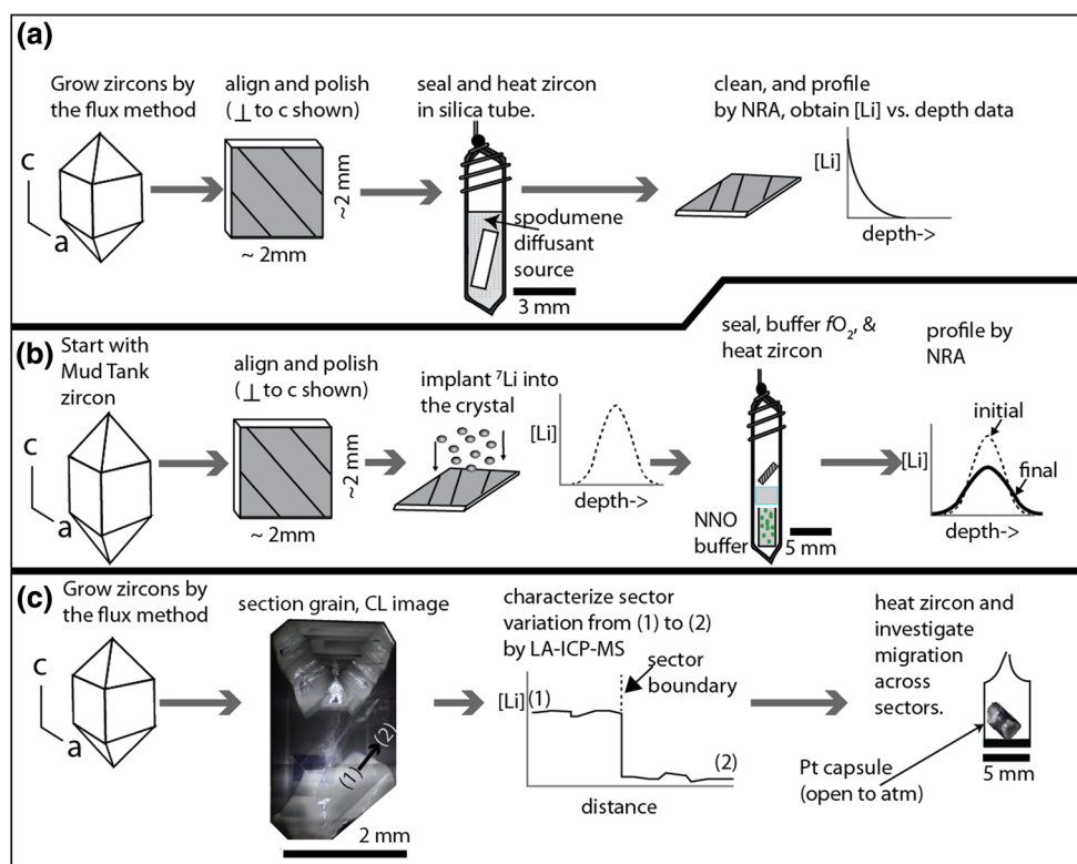
Fig. 1 Overview of the experimental setup for the three types of diffusion experiments conducted here. The CL image shown in (c) is from the actual grain investigated in this study
