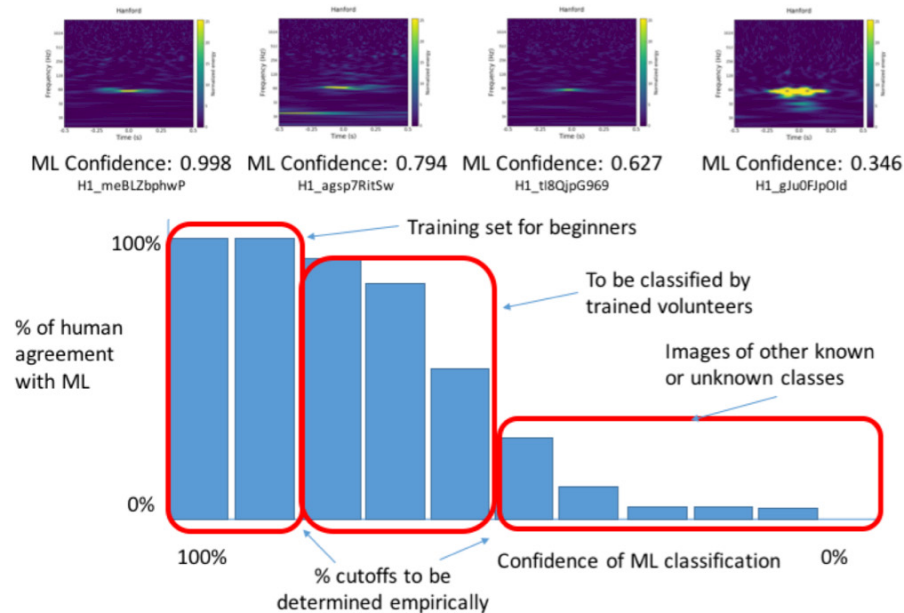
Figure 1. Relationship between ML confidence (x-axis) in a glitch belonging to a class and proportion of images assessed by human exports as belong to that class, with examples of glitches in each grouping.
