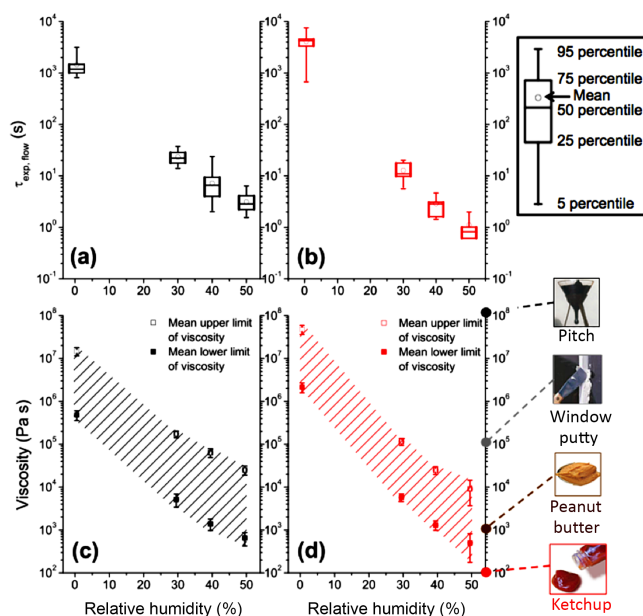
Figure 3. Summary of poke-and-fl w experiments from <0.5 to 50 % RH performed on samples of the whole SOM produced at mass concentrations of 520\ \mu\text{g m}^{-3} (a, c) and 121\ \mu\text{g m}^{-3} (b, d). Panels (a) and (b) show box plots of observed \tau_{\text{exp, fl w}} times for particles poked at different RHs. Panels (c) and (d) show the simulated lower (filled symbols) and upper (open symbols) limits of viscosity. Y error bars represent 95 % confidence intervals, and x error bars represent the range of RH at which measurements were made. The shaded regions are included to guide the eye of the reader. The viscosities of common substances at room temperature have been added to (a) to provide points of reference, as per Koop et al. (2011). The image of pitch is part of an image from the pitch drop experiment (image courtesy of Wikimedia Commons, GNU Free Documentation License, University of Queensland, John Mainstone).
