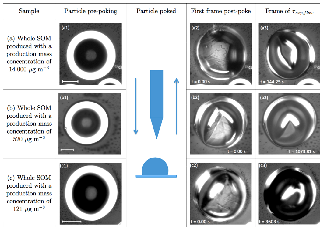
Figure 4. Optical images recorded during typical poke-and-fl w experiments of particles of the whole SOM produced at production mass concentrations of (a) 14\,000\,\mu\text{g m}^{-3} , (b) 520\,\mu\text{g m}^{-3} , and (c) 121\,\mu\text{g m}^{-3} being poked at <0.5\% RH. Panels (a1), (b1) and (c1) correspond to SOM prior to poking. Panels (a2), (b2) and (c2) correspond to the first frame post-poke (i.e. the first frame after the needle has been removed). Panels (a3), (b3) and (c3) correspond to images of the experimental fl w time, \tau_{\text{exp, fl w}} , the point at which the diameter of the hole at the centre of the torus has decreased to 50 % of its original size. Scale bar in panels (a1), (b1) and (c1): 20\,\mu\text{m} .
