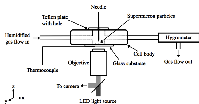
Figure 1. Schematic representation of poke-and-fl w experimental setup.
