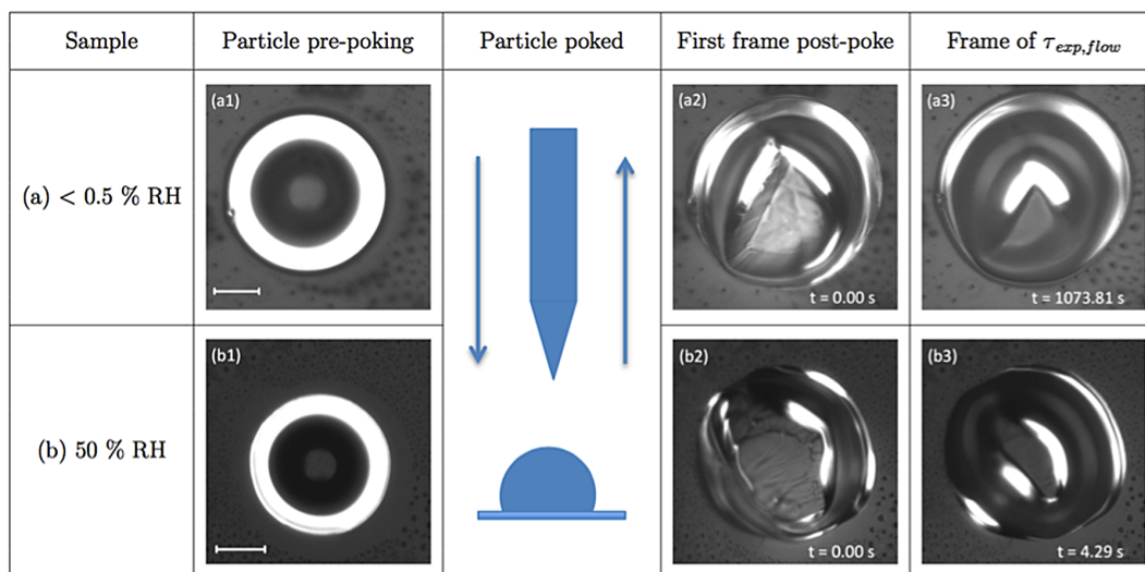
Figure 2. Optical images recorded during typical poke-and-fl w experiments of whole SOM produced at a production mass concentration of 520 \mu\text{gm}^{-3} being poked at (a) < 0.5 \% , and (b) 50 \% , RH. Panels (a1) and (b1) correspond to SOM prior to poking. Panels (a2) and (b2) correspond to the first frame post-poke (i.e. the first frame after the needle has been removed). Panels (a3) and (b3) correspond to images of the experimental fl w time, \tau_{\text{exp, fl w}} , the point at which the diameter of the hole at the centre of the torus has decreased to 50 % of its original size. Scale bar in panels (a1) and (b1): 20 \mu\text{m} .
