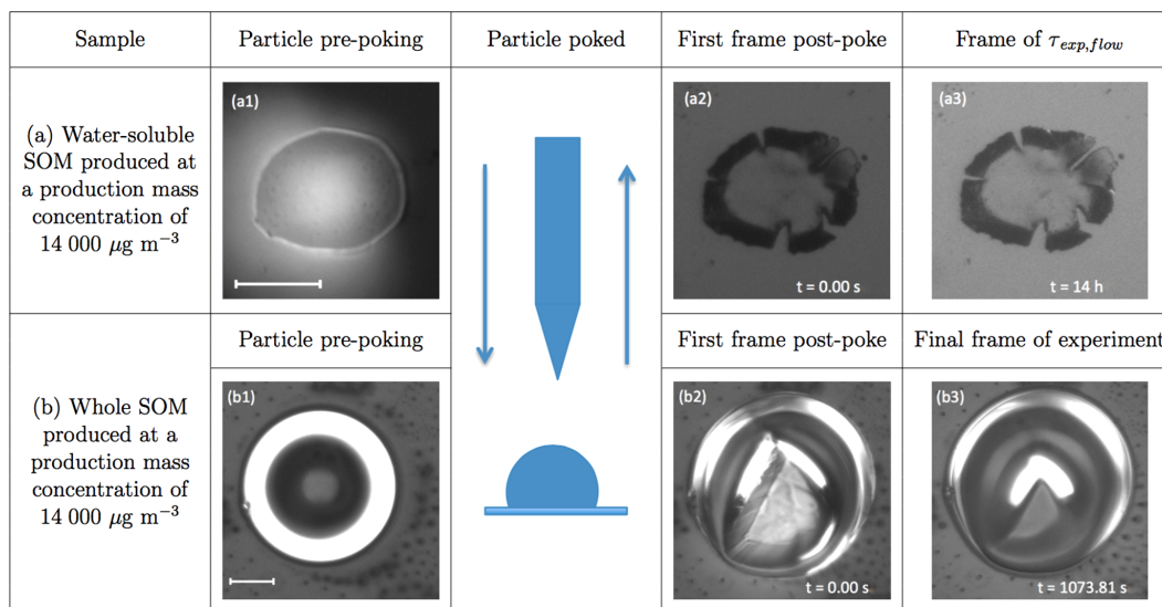
Figure 6. Optical images recorded during poke-and-fl w experiments using particles consisting of (a) the water-soluble component of the SOM and (b) the whole SOM (i.e., both the water-soluble and the water-insoluble components). In both experiments the SOM was produced using a mass concentration of 14\,000\,\mu\text{g m}^{-3} and was poked at <0.5\% RH. Panels (a1) and (b1) correspond to the SOM prior to being poked. The brightness in panel (a1) is due to reflection of the source light by the needle positioned just above the particle. Panels (a2) and (b2) correspond to the first frame post-poke (i.e. the first frame after the needle has been removed). The particle comprised of the water-soluble component of SOM exhibited cracking behaviour and, as shown in panel (a3), no change in the size or shape of the cracks can be observed 14 h after the particle has been poked. The particle comprised of whole SOM exhibited fl w, and panel (b3) corresponds to an image of the particle at its experimental fl w time, \tau_{\text{exp, fl w}} , the point at which the diameter of the hole at the centre of the torus has decreased to 50 % of its original size. Scale bar in panels (a1) and (b1): 20\,\mu\text{m} .
