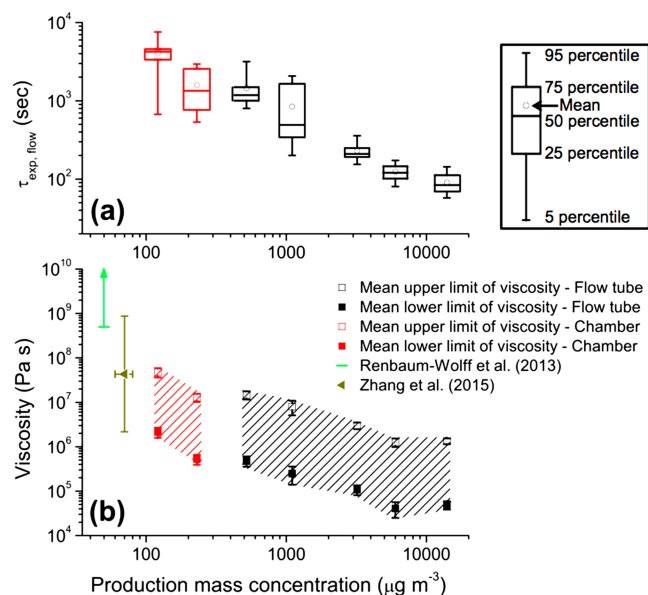
Figure 5. Summary of poke-and-fl w experiments performed on samples of whole SOM at <0.5\% RH. Black symbols represent results from particles produced in a fl w tube, whilst red symbols represent results from particles produced in a chamber. Panel (a) shows box plots of observed \tau_{\text{exp, fl w}} times at different production mass concentrations for particles poked <0.5\% RH. Boxes represent the 25, 50, and 75 percentiles, open circles represent median values, and whiskers represent the 5 and 95 percentiles. Panel (b) shows the simulated lower (filled squares) and upper (open squares) limit of viscosity for particles at each production mass concentration poked at <0.5\% . Symbols represent mean values. The y error bars represent 95 % confidence intervals. The shaded regions are included to guide the eye of the reader. Also included in (b) are literature viscosities for SOM produced via the ozonolysis of \alpha -pinene (Renbaum-Wolff et al., 2013; Zhang et al., 2015).
