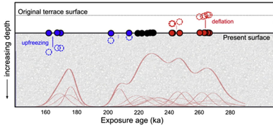
Fig. 7. A cartoon depicting our explanation of the observed scatter in the outwash cobble exposure ages viewed as a cross-section through the terrace. The y-axis displays depth within the terrace sediment, while the x-axis shows age. Also shown are the camel plots and exposure ages of the measured cobbles (solid circles) collected from the present-day surface (solid horizontal line). Thin lines are individual ages and thick lines the summed probability. The original depositional surface (dotted line) has deflated through time to the present day position. The bulk of outwash cobbles have remained in situ (black), which corresponds with the peak in the camel plot. However, several surface cobbles remained on the surface or became exposed as the surface lowered (red), while others have been brought to the surface through cryoturbation (blue). We infer terrace erosion rates of \sim 0.5 \text{ m Ma}^{-1} (Hein et al., 2009) equating to about 14 cm of surface lowering. Measurements of soil depth are 10–15 cm, suggesting upfreezing is likely limited to the upper surface. (For interpretation of the references to colour in this figure legend, the reader is referred to the web version of this article.)
