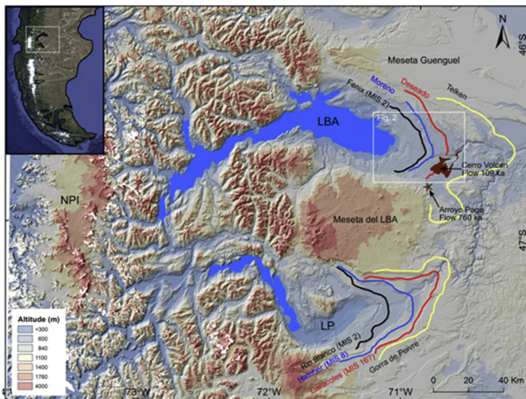
Fig. 1. The figure shows the location of the field site in central Patagonia and the present-day North Patagonian Icefield (NPI). The over-deepened Lago Pueyrredón (LP) and Lago Buenos Aires (LBA) valleys were conduits for major outlet glaciers of the Patagonian Ice Sheet. The figure shows the approximate position of the key moraine limits preserved in each valley, their approximate age and Marine Isotope Stage (MIS), and other geographical information. The present study aims to validate the morphostratigraphic relationships for the penultimate Moreno/Hatcher moraine systems. The figure is derived from Shuttle Radar Topography Mission (SRTM) 30 m digital elevation model (DEM). The inset shows the location in southern South America.
