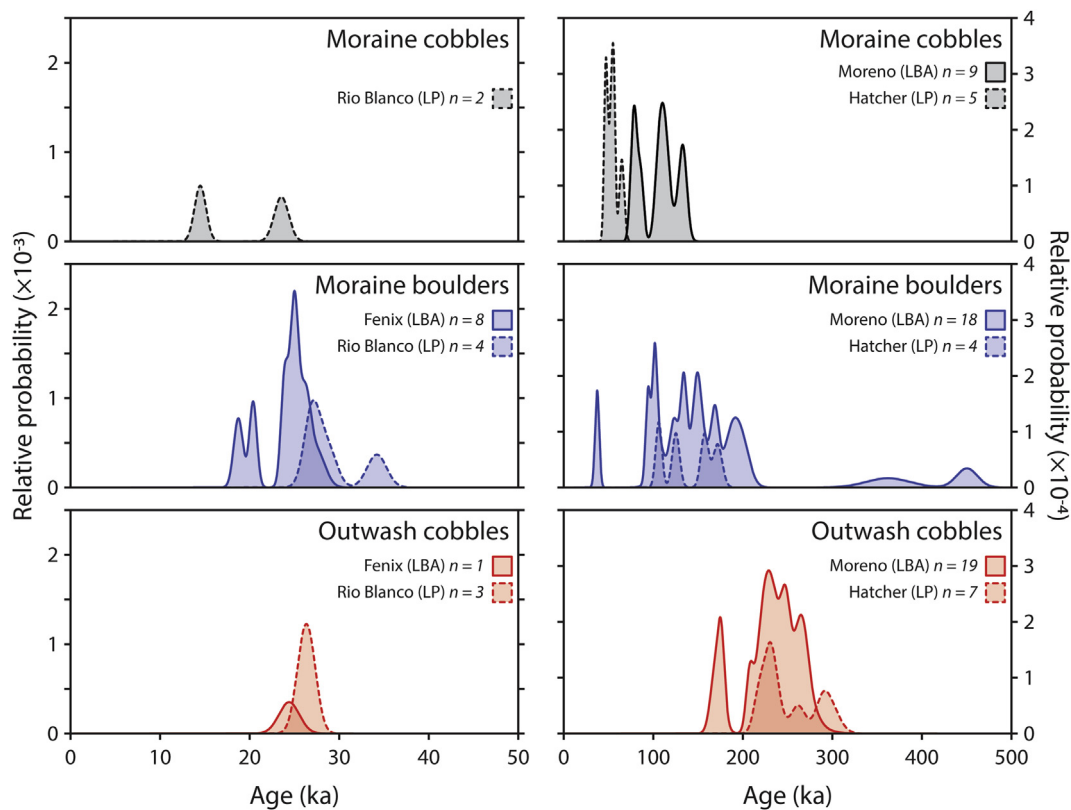
Fig. 8. Comparison of exposure ages between the Lago Buenos Aires (LBA; solid lines) and Lago Pueyrredón (LP; dashed lines) valleys. The camel plot shows all exposure ages (including outliers) obtained from outwash cobbles (red), moraine boulders (blue) and moraine cobbles (black) for the Moreno and Hatcher systems (right), and the Fenix and Río Blanco systems (left). We note that boulders from Moreno III (which include the two oldest) are clumped together with boulders from Moreno I and II; this might not be appropriate since the Moreno III moraine may be older. Exposure ages are indistinguishable between the two valleys and suggest an LGM age for the Fenix/Río Blanco systems. For the Moreno and Hatcher systems, moraine boulders and outwash cobbles yield consistently differing ages within each valley. We infer that moraine cobbles reflect moraine degradation, which is not spatially uniform given that moraine cobble exposure ages are slightly younger in the LP valley. The data for the LBA valley are in Tables 1 and 2, while the data from the LP valley are from Hein et al. (2009). (For interpretation of the references to colour in this figure legend, the reader is referred to the web version of this article.)
