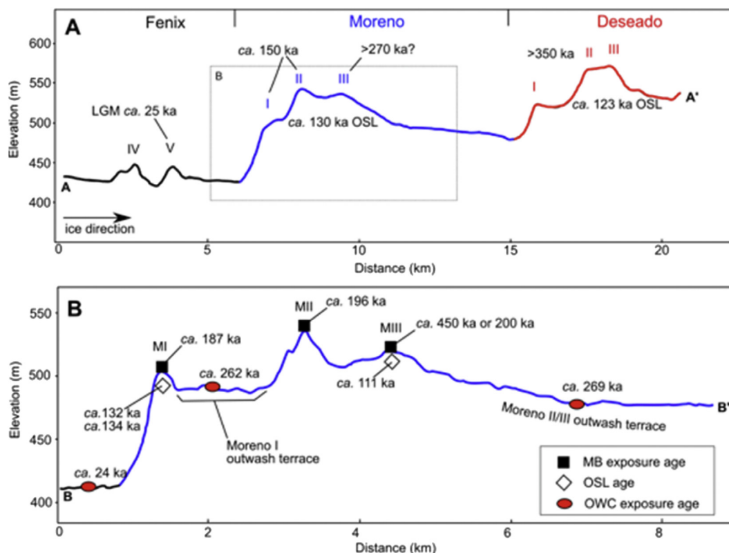
Fig. 3. Surface profiles across the moraine sequences at Lago Buenos Aires. A) Profile showing surface elevation change along the A-A' line in Fig. 2. The figure shows the key moraine sequences and individual moraine limits (numbered). The approximate ages for the landforms are shown based on existing (not re-calculated) cosmogenic nuclide data from moraine boulders (Douglass et al., 2006; Kaplan et al., 2005) and OSL data (Smedley et al., 2016). The figure illustrates the distinct scarps that separate the different glacial sequences. B) The profile shows surface elevation change along the B-B' line in Fig. 2, which cuts across the Moreno system. The figure shows the three Moreno moraine limits (MI–III) and recalculated exposure ages for the oldest moraine boulders (MB) from each (for Moreno III we also include the oldest of two apparent 'outliers'), the OSL ages, and the oldest outwash exposure ages (OWC) from this study. Uncertainties are not shown but are available in Table 2. The figure illustrates how the older Moreno I outwash terrace is situated inboard of and topographically lower than the apparently younger Moreno II/III moraines. We argue the Moreno II/III moraines could not be younger than ca. 260 ka, the age of the Moreno I outwash terrace. Likewise, agreeing with prior studies (Kaplan et al., 2005), we argue the Deseado moraine system cannot be younger than ca. 260 ka. In both figures, former ice direction is left to right. The profiles were extracted from a Shuttle Radar Topography Mission 30 m digital elevation model.
