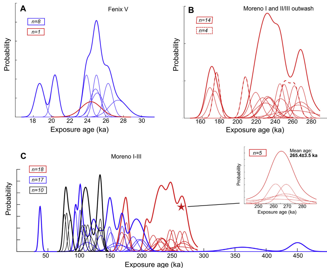
Fig. 6. Camel plots showing ^{10}\text{Be} exposure ages and internal uncertainties for different sample types on the Fenix V and Moreno I–III moraine systems ( n = the number of samples making up each group of data). Note the area beneath each individual Gaussian curve is the same, thus their height is inversely proportional to the measurement uncertainty. A) Plot showing all of the sampled Fenix V moraine boulders (blue) and the single outwash cobble (red). The single outwash cobble gives an LGM age that is indistinguishable from the moraine boulder ages; this is argued to suggest moraines and outwash sediment are deposited with few inherited nuclides. Douglass et al. (2006) did infer the two youngest ages were outliers. B) Plot showing the samples from Moreno I outwash (dashed lines) and the Moreno II/III outwash (solid lines). Both terrace surfaces have a similar age range, suggesting they were deposited at approximately the same time. The multiple peaks are suggestive of geomorphological processes affecting the exposure age results. C) Plot showing all Moreno outwash cobbles (red), moraine boulders (blue) and moraine cobbles (black) together. The figure illustrates how the exposure age is dependent on the nature of the sample and the sample location, including which moraine (Moreno III is stratigraphically the oldest). In general, outwash cobbles are consistently older than moraine boulders while moraine cobbles are the youngest. We argue episodic moraine degradation and rock surface erosion is responsible for the consistently younger moraine exposure ages. The inset shows a camel plot of the five oldest outwash cobble exposure ages making up the oldest peak in the combined camel plot (red star); we take the mean and standard deviation as our preferred age interpretation for the Moreno moraine system. (For interpretation of the references to colour in this figure legend, the reader is referred to the web version of this article.)
