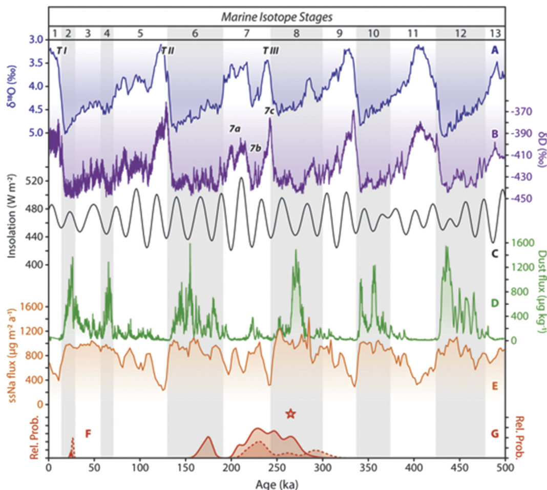
Fig. 9. A comparison of the timing of outwash deposition in LBA and LP with a range of palaeoclimate proxies. (A) The LR04 benthic foraminiferal stack (Lisiecki and Raymo, 2005), which is essentially a proxy for northern hemisphere ice volume. (B) Deuterium record from the Antarctic EPICA Dome C ice core as a proxy for Southern Hemisphere temperature changes (Jouzel et al., 2007). (C) Summer (December) insolation intensity at 50S (Berger and Loutre, 1991). (D) Aeolian dust flux record from the EPICA Dome C ice core (Lambert et al., 2008). (E) Sea salt Na flux as a proxy for Antarctic sea ice variability (Wolff et al., 2006). (F and G) Our ^{10}\text{Be} data for outwash cobbles from LBA (solid lines) and LP (dashed lines) for the Fenix and Río Blanco limits (F) and Moreno and Hatcher limits (G), respectively (F and G plotted on separate relative probability scales). The star shows the timing of Moreno deposition at 260–270 ka. Also shown are the timings of glacial terminations (TI to TIII) and MIS 7a–c, mentioned in the text. The vertical bands correspond with marine isotope stages.
