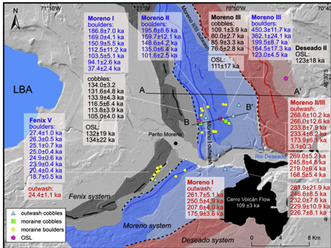
Fig. 2. The Lago Buenos Aires field site and sample locations. The figure shows the key moraine systems with darker shades corresponding to areas dominated by moraine-till, and lighter shading to areas dominated by outwash sediments. The sample locations, ages and analytical uncertainties for each sample type are shown (see Tables 1 and 2 for full sample details). The A-A' line and B-B' line are the profiles shown in Fig. 3. All previously reported exposure ages have been re-calculated to be consistent with the present study (see Section 3.3). The moraine boulder exposure ages from the Fenix moraines are from Douglass et al. (2006) and Kaplan et al. (2004), and for the Moreno moraines, Kaplan et al. (2005). Moraine cobbles exposure ages from Moreno I are from Hein et al. (2009), and from Moreno II/III are from this study, OSL ages are from Smedley et al. (2016), and the ^{40}\text{Ar}/^{39}\text{Ar} age of the Cerro Volcan lava flow is from Singer et al. (2004). All outwash ages are from the present study. The figure is derived from a hill-shaded Shuttle Radar Topography Mission 30 m digital elevation model. (For interpretation of the references to colour in this figure legend, the reader is referred to the web version of this article.)
