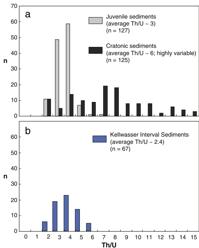
Fig. 6. (a) Th/U ratios in modern sediments showing sedimentary provenance, where clustered Th/U ratios ~3 indicate a juvenile sediment source (after Carpentier et al., 2013), in comparison to more mature cratonic sediments which have higher average Th/U ratios (~6) with more variability. (b) Th/U ratios in the Kellwasser Horizon at the Zhulumute–Hongguleleng Formation boundary cluster ~2.4, indicating a juvenile sediment source, consistent with an island arc.
