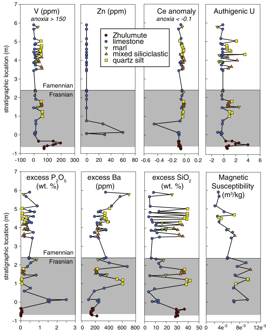
Fig. 9. Geochemical anoxia proxy signatures in the topmost Zhulumute and basal Hongguleng Formations. The Kellwasser interval is shown in gray with the Frasnian–Famennian boundary located 2.4 m above the base of the Hongguleng Formation (see Fig. 3 for relation to stratigraphic section). Although the Kellwasser Event (shaded interval) cannot be detected visually by a change in mineralogy, it can be detected by geochemical proxies such as V/Cr ratios in siliciclastics, Zn concentrations in carbonates, Ce anomalies in phosphate-rich units, and authigenic U content in siliciclastics (Pujol et al., 2006; Tribouillard et al., 2006). Excess whole rock P_2O_5 , Ba, and SiO_2 (Pujol et al., 2006) indicate increased primary productivity in the aftermath of anoxia. Magnetic susceptibility (MS) shows a distinct negative trend, which starts just below the Frasnian–Famennian boundary and is consistent with sea level rise associated with the Kellwasser Event.
