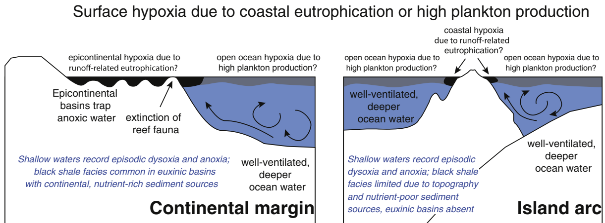
Fig. 12. New model for the Kellwasser Events invoking eutrophication and enhanced surface productivity as a causal mechanism for episodic dysoxia and sustained anoxia, both along continental shelves (model modified from Bond et al., 2004), and along island arc coastlines in the open ocean (model modified from a topographic transect across the Marianas Islands, commonly used as a modern analogue for the Late Devonian tectonic setting of the Hongguleleng Formation).
