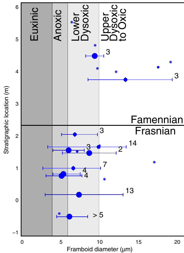
Fig. 11. The size and variability of pyrite frambooids can be used to assess redox conditions (Wignall and Newton, 1998; Bond and Wignall, 2010). Euxinia produces populations of tiny frambooids ( <5 \mu\text{m} ) with a narrow size range. In dysoxic environments the frambooids are larger and more variable in size ( 5\text{--}15 \mu\text{m} ). Frambooids are rare in oxic environments. The chart shows the distribution of frambooids from SEM. Individual points indicate a single frambooid in the sample. Lines show minimum, maximum and average size for the frambooid population in that sample. Frambooid populations are indicated for each large data point where n > 1 . Based on the frambooid populations, the Upper Frasnian shows an anoxic to lower dysoxic environment consistent with the Kellwasser Anoxia Event. Frambooids are much less abundant in the Famennian part of the section indicating a change to upper dysoxic to oxic environments. Stratigraphy is measured from the base of the Hongguleleng Formation.
