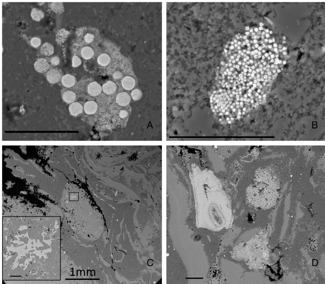
Fig. 10. Backscattered scanning electron microscope photomicrographs of (A) Late Frasnian pyrite framboids from 0.74 m above the base of the Hongguleleng Formation; (B) lower Famennian Fe oxide aggregates from 4.0 m above the base of the Hongguleleng Formation; (C) pore-filling apatite (light gray color) in pore spaces between brachiopod shells and filling voids in peloid interiors (inset box), indicating a non-detrital dissolved phosphate source within the water column; and (D) microbially mediated apatite (light gray, porous grains in the top right and center bottom), in contrast to a broken conodont in the top left. Scales are 50 \mu except as noted.
