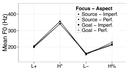
Figure 1: Mean F0 values for each tone in the L+H* L-H% contours, for the contrastively focused region in each critical condition.
