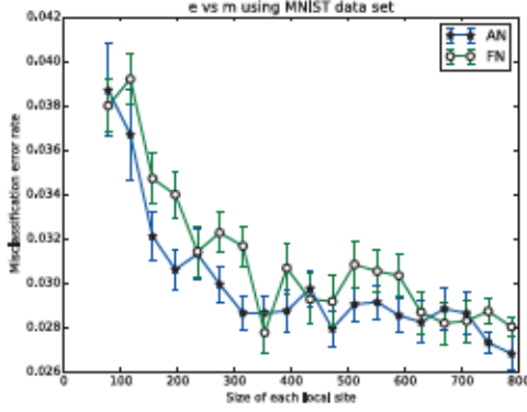
Fig. 1. e vs. m , non-private for MNIST
