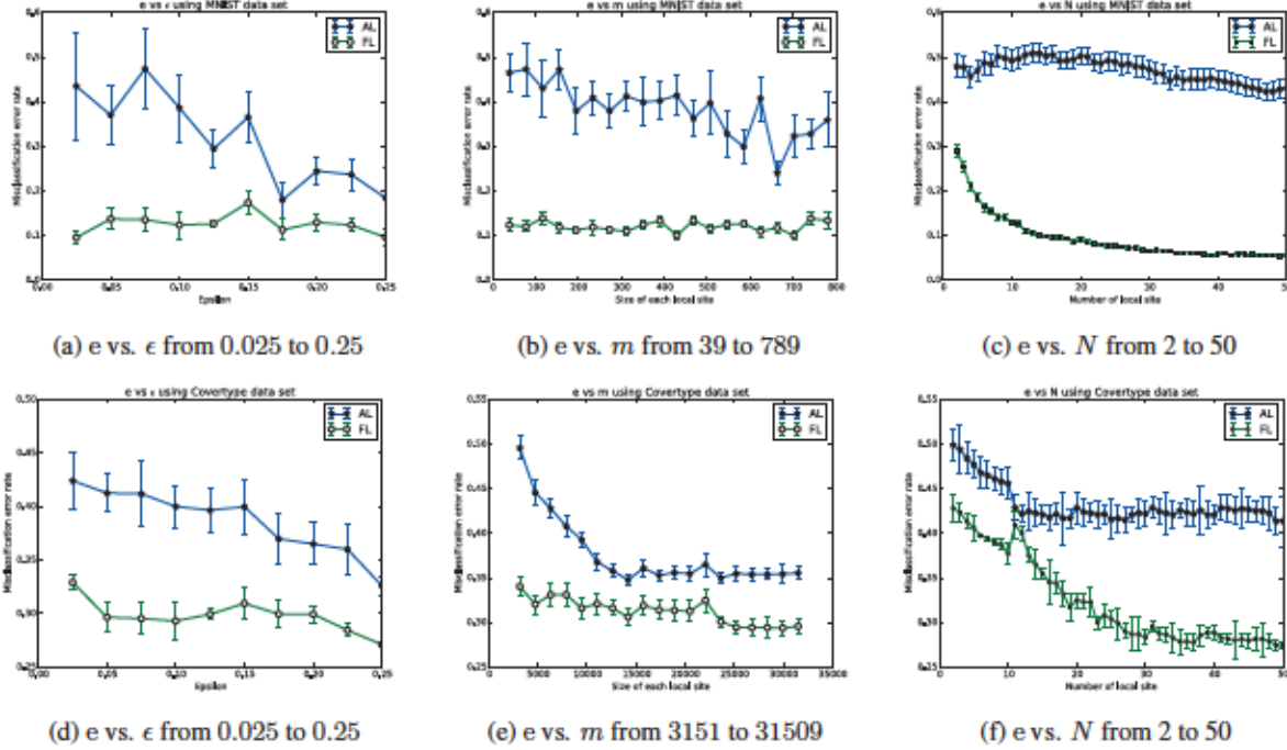
Fig. 3. Performance of algorithms for MNIST (top row, \Lambda = 10^{-2} ) and Covertype (bottom row, \Lambda = 10^{-7} ) for N = 10 , h = 0.5 . Error e versus \epsilon \in [0.025, 0.25] (3a,3d), m (3b from 39 to 789, 3e from 3151 to 31509), and N (3c,3f)
