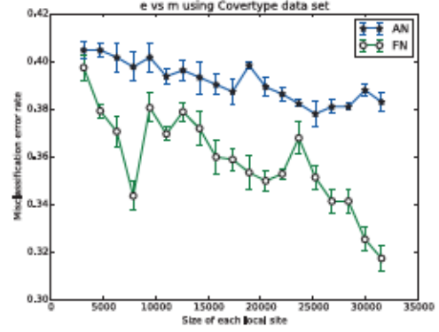
Fig. 2. e vs. m , non-private for Covertypes
