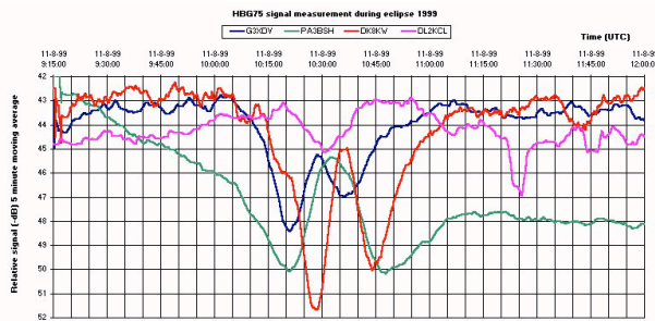
Figure 3. Relative signal strength from HBG Switzerland at 75 kHz during 1999 solar eclipse. https://misan.home.xs4all.nl/eclipse.htm
