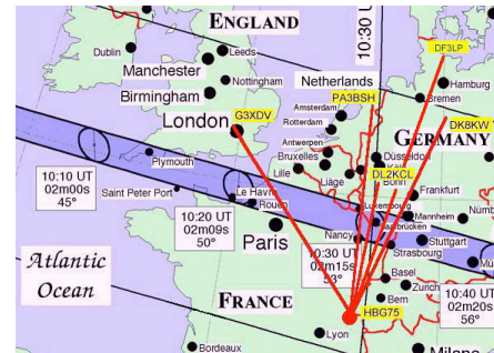
Figure 3. Relative signal strength from HBG Switzerland at 75 kHz during 1999 solar eclipse. https://misan.home.xs4all.nl/eclipse.htm
