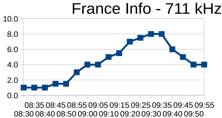
Figure 2. Received signal strength (in S units) at Wolverhampton, UK vs time (left) and eclipse path (right) for the transmitter located south of Wolverhampton at Rennes-Thourie, France [2]. Map from NASA shows the eclipse path.
