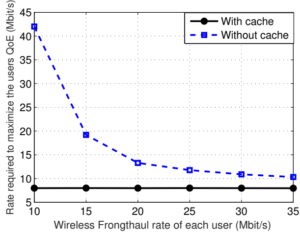
Fig. 6. Rate required to maximize the users QoE as the fronthaul rate of each user changes.
