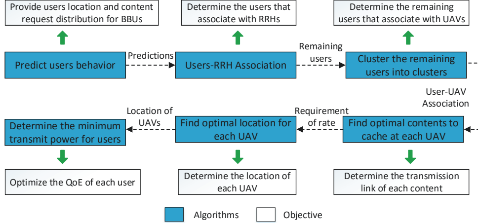
Fig. 2. The procedure used for solving the optimization problem given in (19).
