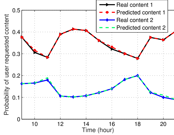
Fig. 4. Content request probability predictions.
