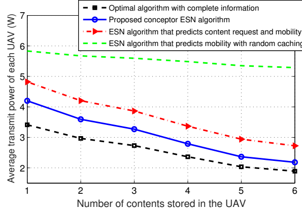
Fig. 9. Average minimum transmit power as the number of the contents stored in a UAV cache varies ( U = 70 and K = 5 ).
