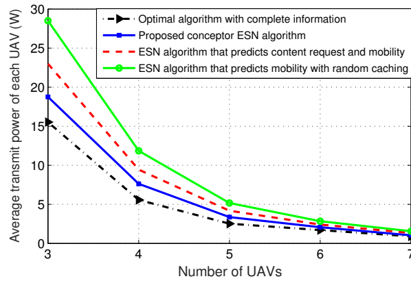
Fig. 8. Average minimum transmit power as the number of UAVs changes ( U = 70 and C = 1 ).
