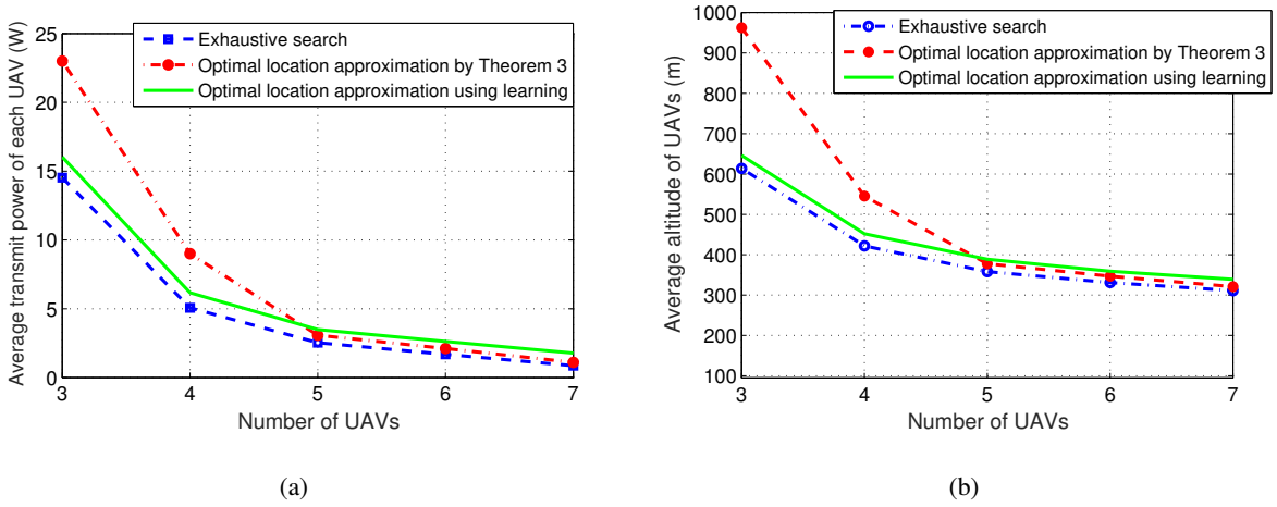
Fig. 10. Average minimum transmit power and average altitude vs. the number of the UAVs.
