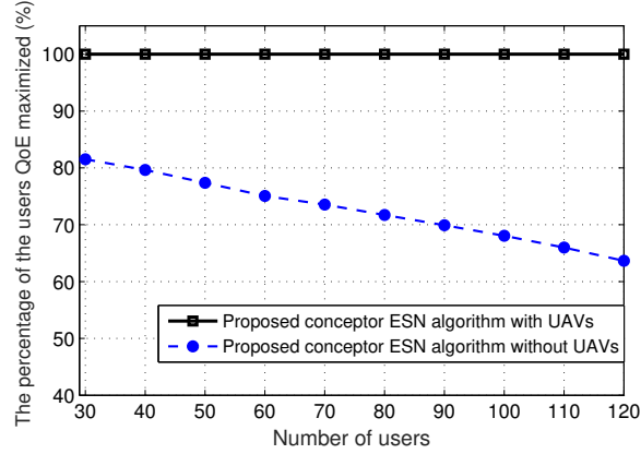
Fig. 7. The percentage of the users QoE that is maximized as the number of the users varies
