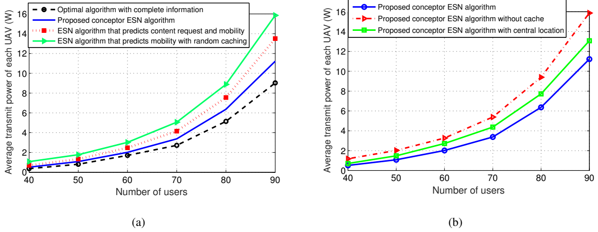
Fig. 5. Average minimum transmit power as the number of the users varies. ( K = 5 and C = 1 .)
