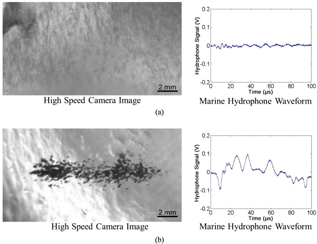
Fig. 4. Example waveforms collected by marine hydrophone with corresponding optical images of bubble cloud. Results show a significant increase in the amplitude of the waveform collected by the marine hydrophone when a cavitation cloud has been initiated compared with uninitiated cases. Examples shown are of 2.5% agarose tissue phantoms treated at 10 Hz right below and above the cavitation cloud threshold with peak negative pressures of (a) 24.2 MPa and (b) 25.1 MPa. The threshold for cloud initiation was determined to be the lowest pressure at which a bubble cloud was initiated within ten pulses and maintained for the duration of the treatment for all six samples.
