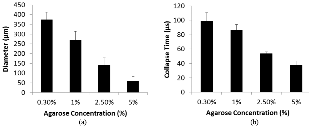
Fig. 8. Bubble expansion in agarose tissue phantoms of varied concentration. Results show the maximum bubble expansion and the bubble collapse time for bubbles produced by histotripsy in agarose tissue phantoms. Results show a significant decrease in (a) maximum bubble expansion and (b) bubble collapse time with increasing agarose concentration. All decreases in bubble diameter and collapse time between gel concentrations were considered significant ( p -values < 0.05 ).
