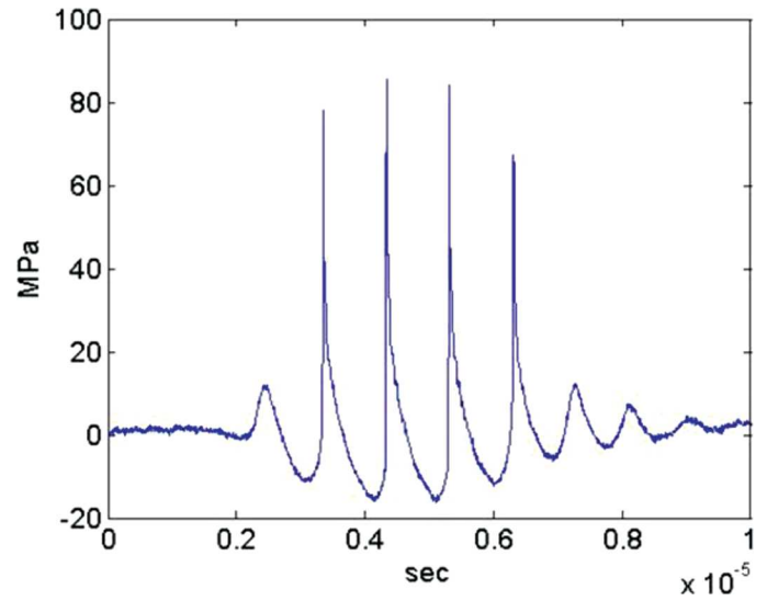
Fig. 3. Example histotripsy pressure waveform.
